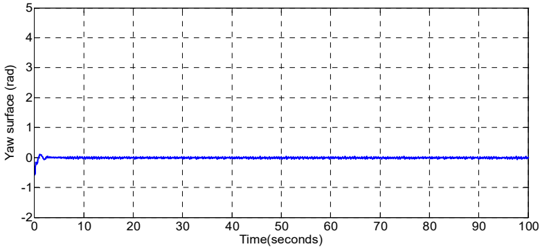
Fig. 9. Yaw surface with matched disturbance given at 50 seconds (non-linear sliding surface design)
