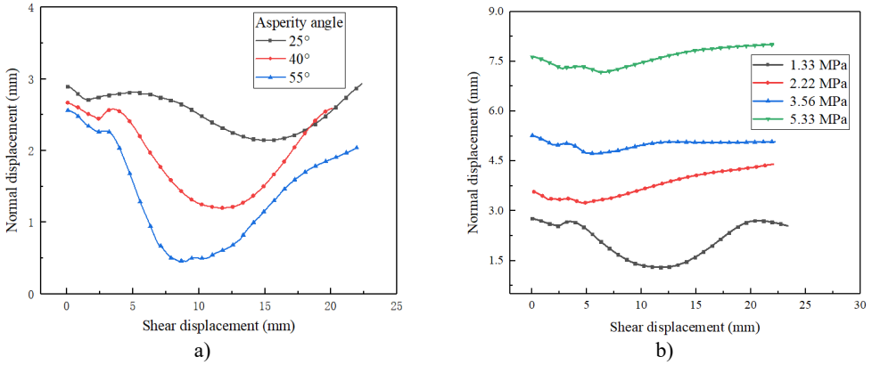
Fig. 9. Typic dilatancy curves: a) asperity angles under the normal stress of 1.33 MPa, b) asperity angle of 40° under different normal stresses
