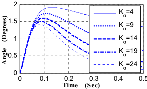
Fig. 6. Pitching angular displacement curves vs. K_\alpha
