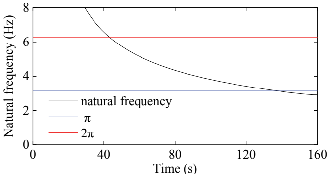
Fig. 8. The first order natural frequencies of the two hoisting ropes corresponding to Fig. 7
