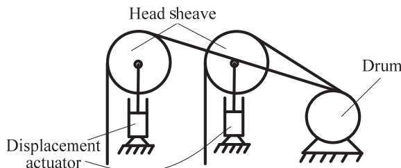
Fig. 12. Schematic of control strategy
