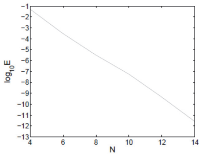
Fig. 3. L^\infty error of Example 2
