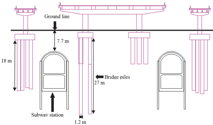
Fig. 3. The bridge piles and the subway station
