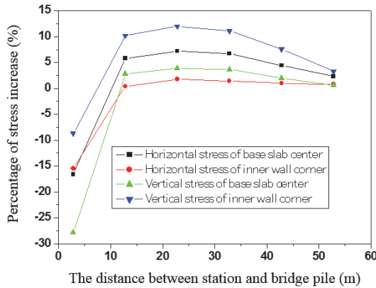
Fig. 8. The relationship between the percentage of stress increase and the distance
