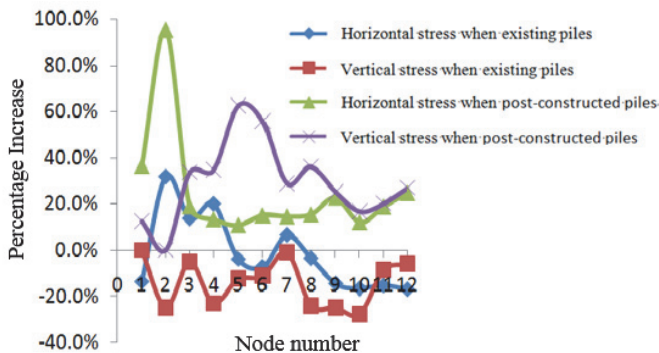
Fig. 4. Stress percentage increase of existing and post-constructed piles compared to that without piles. Node number: 1 – Upper station arch crown center, 2 – Lower arch crown center, 3 – Inner arch foot, 4 – Outer arch foot, 5 – Upper diaphragm slab center, 6 – Lower diaphragm slab center, 7 – Inner diaphragm slab and side wall border, 8 – Outer diaphragm slab and side wall border, 9 – Upper floor center, 10 – Lower floor center, 11 – Inner wall corner, 12 – Outer wall corner
