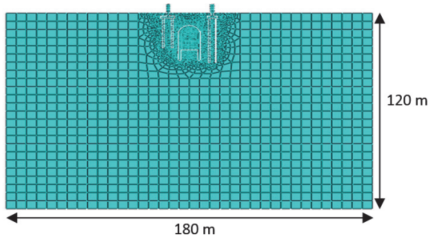
Fig. 2. A two-dimensional FEM of the structure with piles
