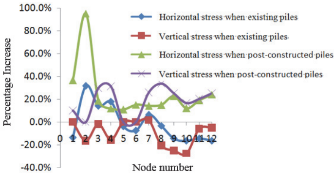
Fig. 5. Stress percentage increase of existing and post-constructed piles compared to that without piles under earthquake excitation. Node number: 1 – Upper station arch crown center, 2 – Lower arch crown center, 3 – Inner arch foot, 4 – Outer arch foot, 5 – Upper diaphragm slab center, 6 – Lower diaphragm slab center, 7 – Inner diaphragm slab and side wall border, 8 – Outer diaphragm slab and side wall border, 9 – Upper floor center, 10 – Lower floor center, 11 – Inner wall corner, 12 – Outer wall corner
