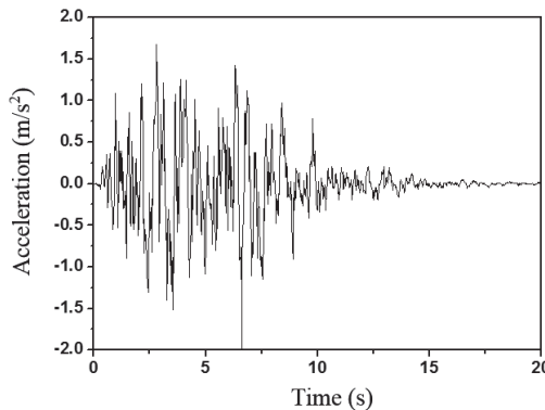
Fig. 1. The time-history curve of artificial earthquake
