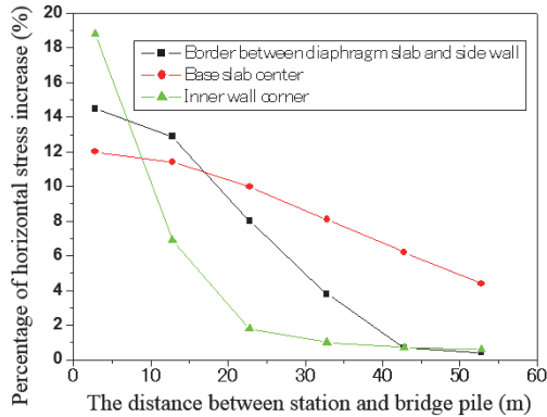
Fig. 6. The relationship between the percentage of horizontal stress increase and the distance
