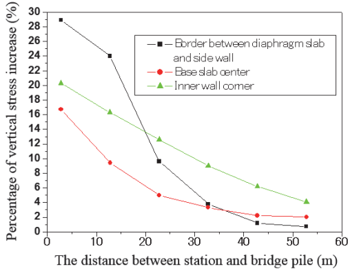
Fig. 7. The relationship between the percentage of vertical stress increase and the distance
