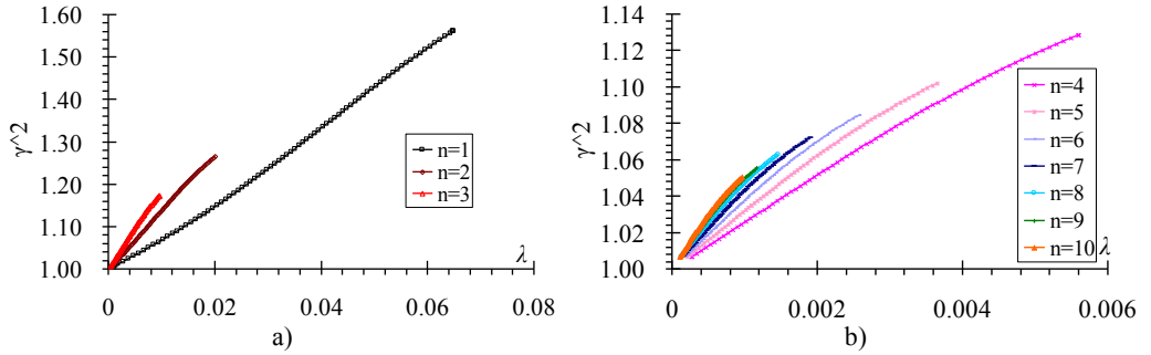
Fig. 4. \gamma_n^2 - \lambda_n relation curves a) n = 1-3 , b) n = 4-10
