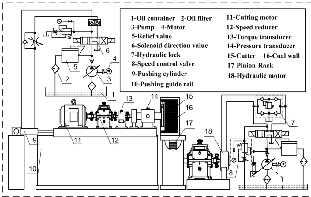
Fig. 12. Revolving cutting test-bed
