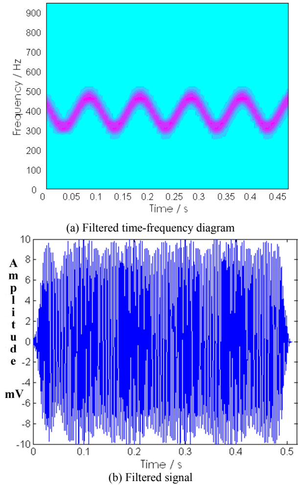
Fig. 3. Result of time-frequency filtering
