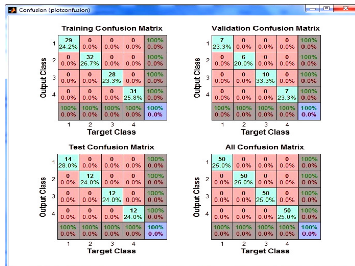
Fig. 7. Confusion matrix
