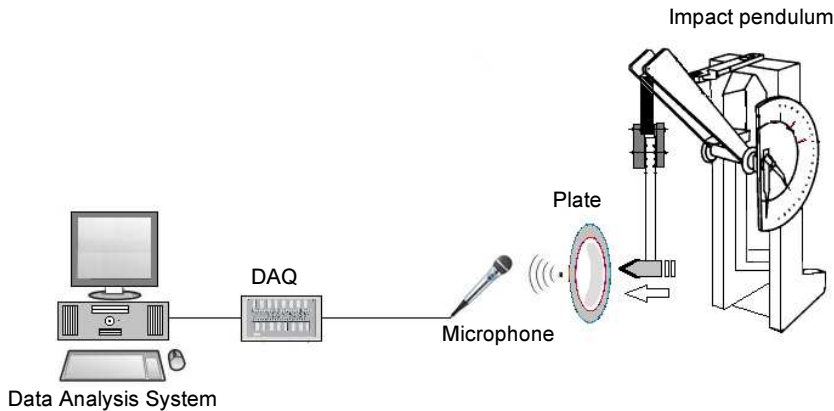
Fig. 1. Data acquisition and measurement system [1]
