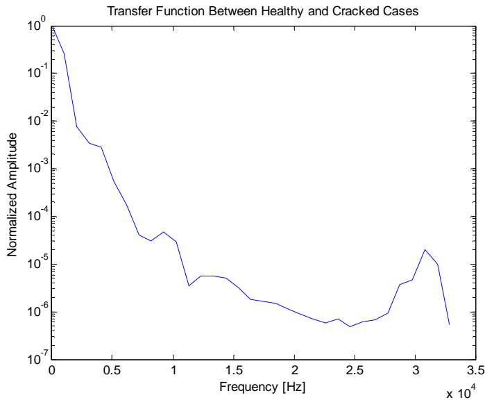
Fig. 6. Transfer function between healthy and cracked cases
