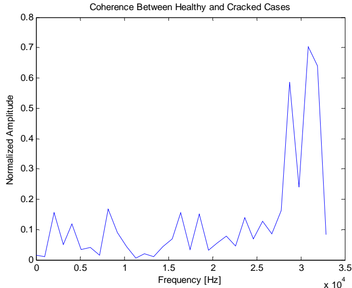
Fig. 5. Coherence between the healthy and cracked cases
