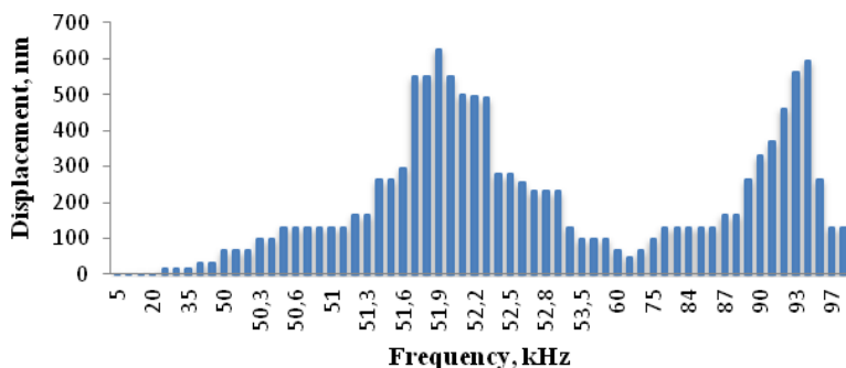
Fig. 4. Dependence of the displacement with respect to frequency (voltage 10 V)
