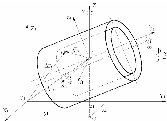
Fig. 1. Calculation scheme
