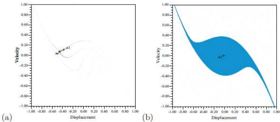
Fig. 11. 2D sections at y = 0 of the 3D basins of attraction for a_0 = 0.1 , \zeta = 0.05 , a_3 = -4 and \beta = 0.05 . (a) \omega = 0.76 ; (b) \omega = 2.50
