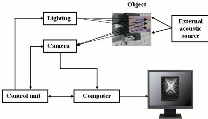
Fig. 3. A structural scheme of the holographic system PRISM
