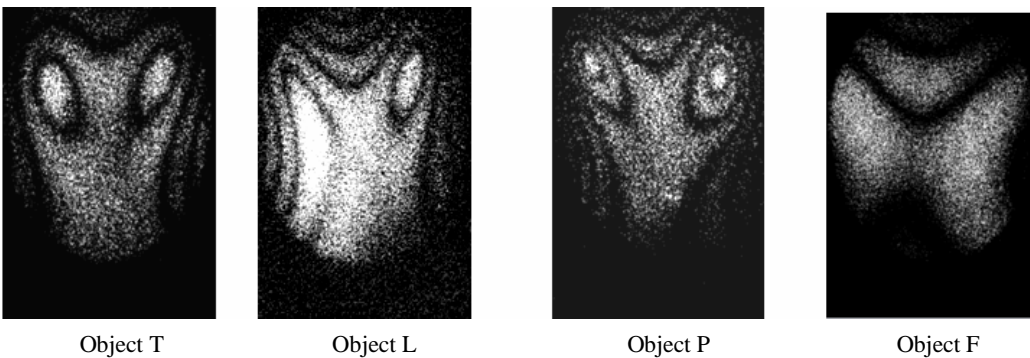
Fig. 7. Interferograms of four objects that have been obtained under external acoustic excitation frequency of 460 Hz
