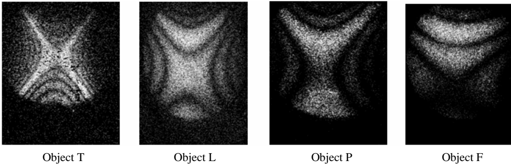
Fig. 5. Interferograms of four objects that have been obtained under external acoustic excitation frequency of 427 Hz
