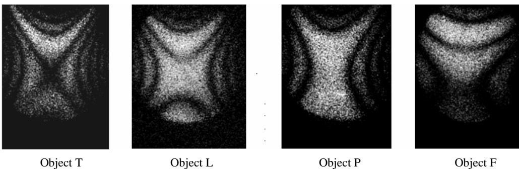
Fig. 6. Interferograms of four objects that have been obtained under external acoustic excitation frequency of 432 Hz
