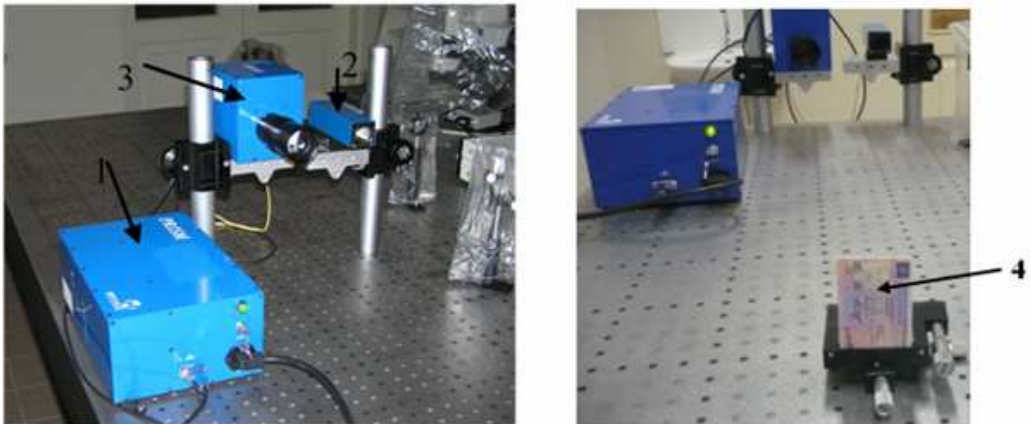
Fig. 2. Holographic system PRISM: 1 – control unit; 2 – source of the object-oriented beam; 3 – camera, 4 – the object to be investigated, namely a driving license (polycarbonate plate with dimensions of 85.7×54.1×0.8 mm)
