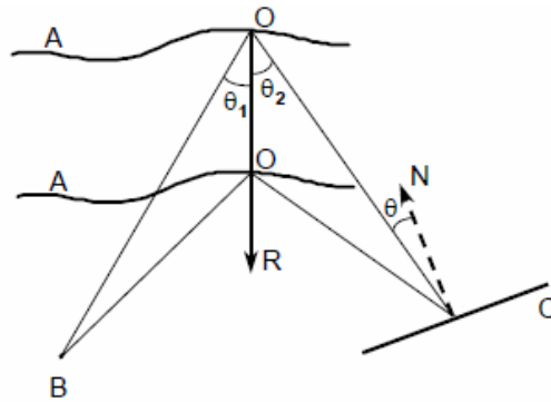
Fig. 1. The scheme of holographic experiment: A – oscillating object; B – laser light source; C – camera; O – point on the surface of the body; R – vector of displacement; N – normal vector of the hologram plate.
