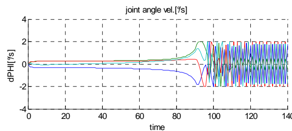
Fig. 8. Joint motion near singularity
