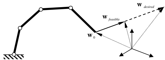
Fig. 1. Affine Manipulability according to [1]
