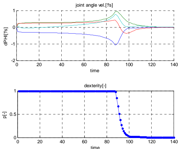
Fig. 9. Dexterity and joint motion near singularity due to limited Lagrange multipliers
