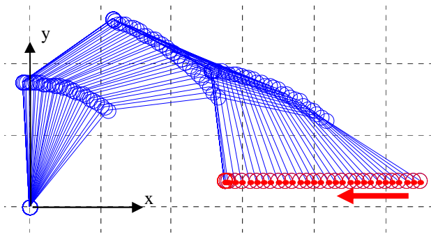
Fig. 5. x-y-motion of the manipulator according to the proposed approach LP2
