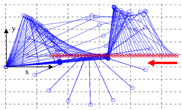
Fig. 3. x-y-motion of the manipulator according to LP1
