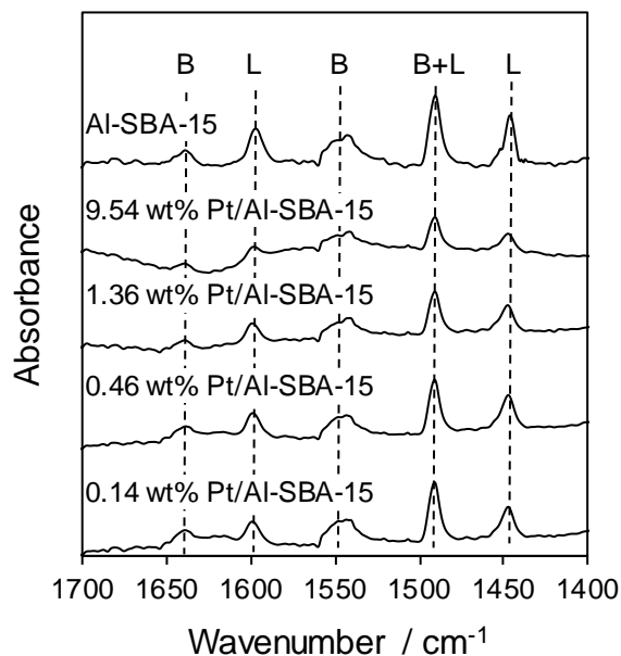
Figure 1. DRIFT spectra of chemisorbed pyridine over Pt/Al-SBA-15.
