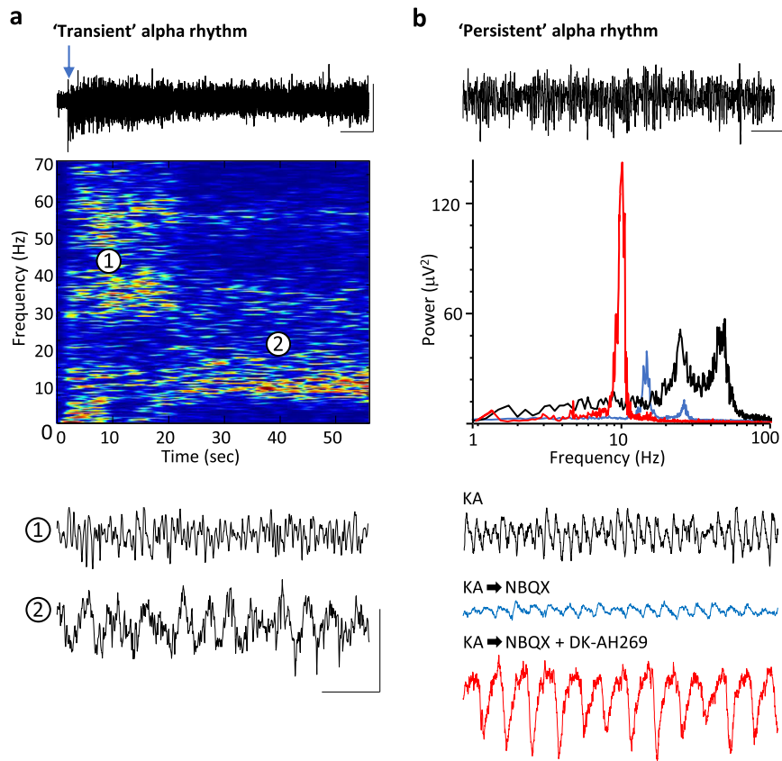
Fig. 1 Alpha rhythms are generated in visual neocortex after transient periods of cellular and network excitation. a Alpha rhythms manifest following glutamate-induced gamma rhythms in slices of V1 under cholinergic (10 \mu M carbachol) neuromodulation. Upper example trace shows 60 s of L4 LFP with glutamate ejected at the time of the arrow. Graph shows an example colormapped spectrogram of the resulting pattern of rhythm generation. Note the initial generation of dual (high- and low-) gamma rhythms, which rapidly transition to a single alpha rhythm at ca. 20 s. Lower example traces show examples from the 2 time points as indicated in the spectrogram. Scale bars upper trace, 100 \mu V, 6 s; lower traces, 100 \mu V, 200 ms. b A pharmacological model, based on the findings in a produced a more 'persistent' alpha rhythm lasting over 160 min. Upper trace shows a 30 s example of alpha rhythms generated pharmacologically. Graph shows example spectra in three experimental conditions: Bath application of kainate alone in the initial, excitatory stage of the model (black) generating dual-gamma spectral peaks; bath application of NBQX and DK-AH269 to generate a robust alpha rhythm (red); bath application of NBQX alone to reduce AMPA receptor-mediated excitation (blue). Lower example traces show examples in each of these three conditions. Scale bars upper trace 100 \mu V, 3 s, lower traces, 100 \mu V, 200 ms.
