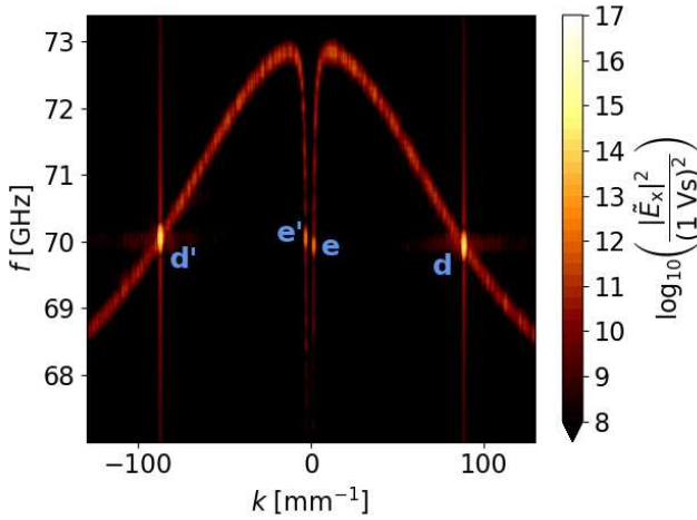
(b) k - and f -space for I_{\text{pump}} = 1 kW/mm 2 and 25 \text{ ns} < t < 35 \text{ ns} like in figure 7b. Bold blue letters are labels for nearby peaks mentioned in the text.
