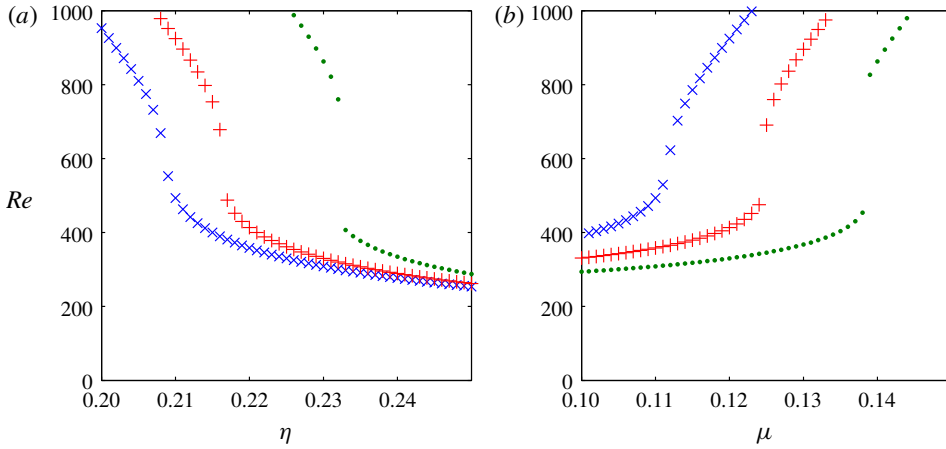
FIGURE 11. Tracking the discontinuity in Re_c near to the point X in figure 2. Each plot shows the critical Reynolds number Re_c for instability for a range of \eta and \mu values. In both plots we have Fr = 1.0 . We can see that the system transitions from continuous to discontinuous as \eta and \mu are increased. In (a), we have 0.2 < \eta < 0.25 . Blue crosses give the results for \mu = 0.11 , red pluses give the results for \mu = 0.12 and green dots give the results for \mu = 0.14 . In (b), we have 0.1 < \mu < 0.15 . Blue crosses give the results for \eta = 0.21 , red pluses give the results for \eta = 0.22 and green dots give the results for \eta = 0.23 .
