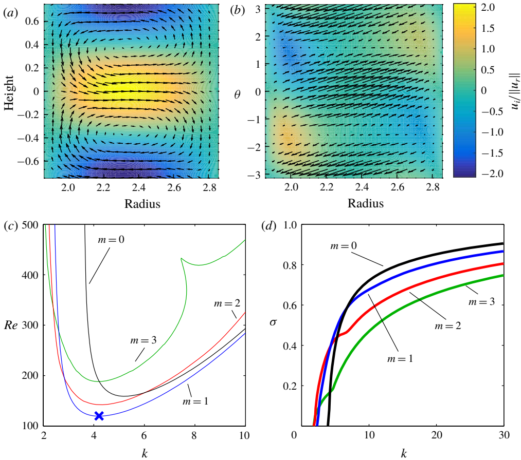
FIGURE 5. See § 5.2 for a description of the multiplot layout. Another example of critical viscous SRI, here for \eta = 0.65 , \mu = 0.25 and Fr = 1.0 , occupying region \beta of figure 2. The critical viscous mode of instability has Re_c = 119.6 with m = 1 , k = 4.208 , and \omega = 0.5246 . For this frequency, \mathcal{R}[\Phi(r_c)] = 0 occurs at r_c = 2.332 . \mathcal{R}[\Phi(r_{\pm})] = \pm\sqrt{2Z\Omega} cannot occur for this (\eta, \mu) because 2Z\Omega < 0 throughout the radial range.
