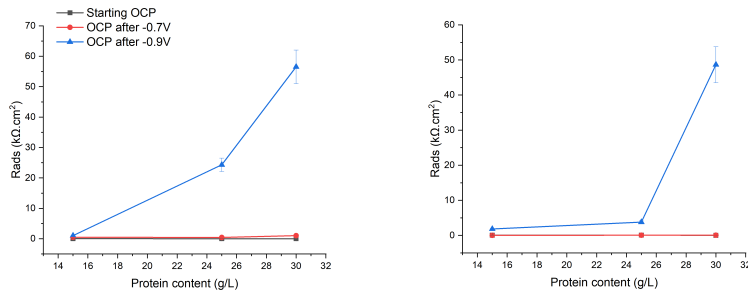
Figure 8 R_{ads} at 37°C (on the left hand) and 50°C (on the right hand) for starting OCP and OCP after cathodic polarization at different protein concentration solutions
