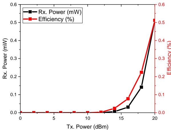
FIGURE 15: Measured output power and RF-DC conversion efficiency of proposed rectenna at 24 GHz as a function of input power at a distance of 0.15 m.
