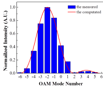
Fig. 4. The distribution of the OAM spectrum when the OAM beam of l_1 = -2 is received by an angular aperture of \pi/2 .
