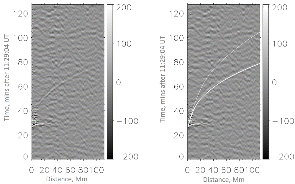
Fig. 8. Time–distance diagram for the seismic source 2, obtained from the filtered HMI dopplergram without (left) and with (right) theoretical curves. The TD diagram shows the ridge derived from ripples produced at some distance from the event location by acoustic waves in their first bounce from the photosphere (lower white line) and the second bounce (upper white line). The start (zero) time on the Y-axis is 11:29.04 UT, which corresponds to the shock deposition and seismic response initiation at 11:55:37 UT. The grey colour bars on the right show the background Doppler velocities in m/s.
