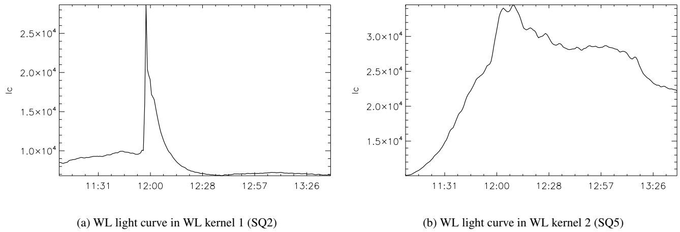
Fig. 15. (a) Temporal profiles of white light emission obtained in the WL kernel 1 in the locations of the H\alpha kernels 2 and seismic source 2, and (b) WL light curve in kernel 2 at the location of H\alpha kernel 3 and possible seismic source 5.
