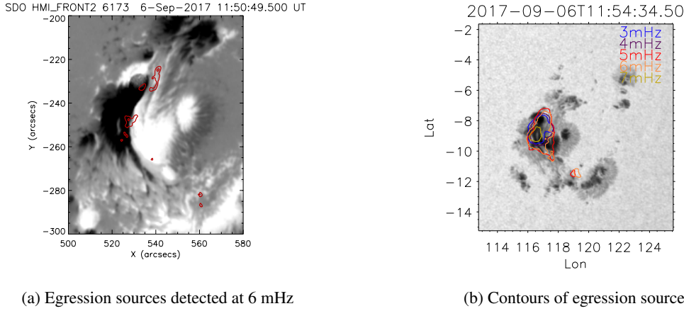
Fig. 4. (a) HMI magnetogram of the active region overplotted with egression maps at 6 mHz only. (b) Contours of the egression maps of sunquakes 1-4 in different frequencies marked by different colours over-imposed on the WL image.
