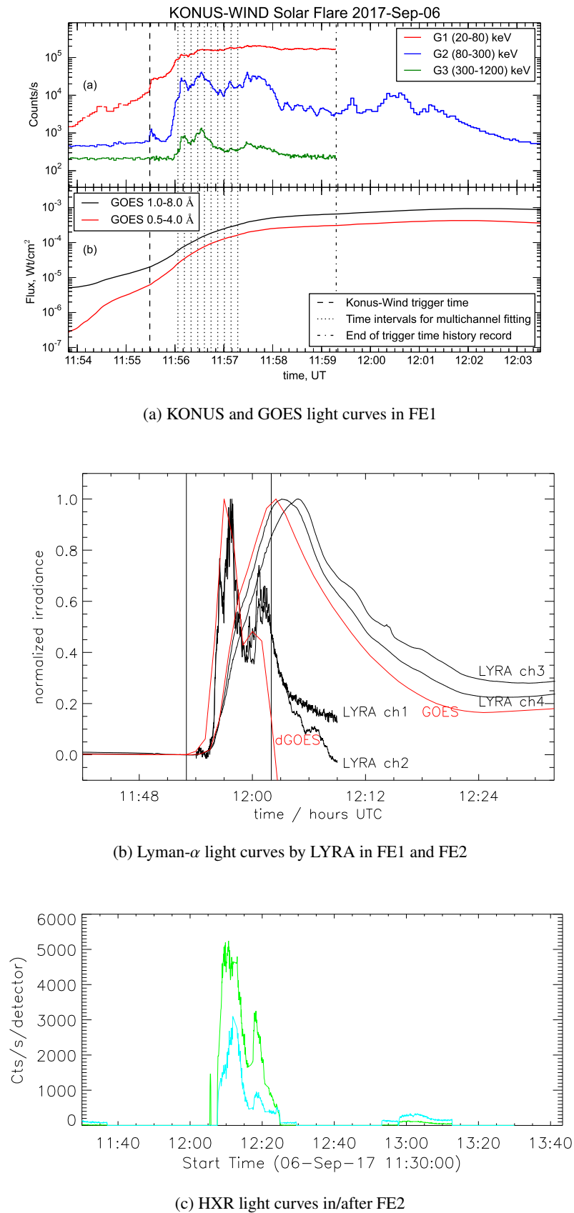
Fig. 2. The light curves of the X9.3 flare. a): Light curves by the KONUS instruments (upper plot) and by GOES (bottom plot). b): the light curve in Ly- \alpha line observed by the LYRA instrument (Hochedez et al. 2006; Dominique et al. 2013) showing flaring events 1 (after 11:55 UT) and 2 (after 12:04 UT, see the text for details). c): the light curves of HXR emission during or after the flaring event 2 observed after 12:08 UT by RHESSI, Green line - 25 - 50 keV; Cyan line: 50 - 100 keV (scaled).
