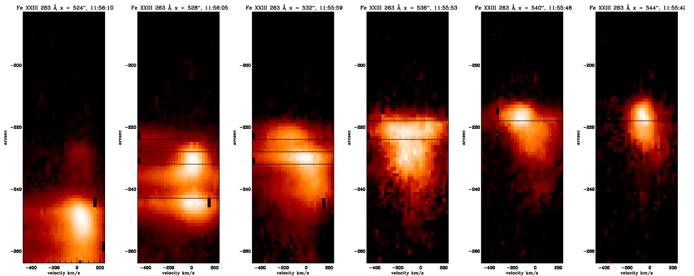
Fig. 13. Flaring event 1 ( >11:55 UT): Series of EIS spectrograms in the Fe XXIII 263.76 \text{ \AA} line taken during the onset phase of the X9.3 flare on 6 September 2017. The titles above spectrograms indicate the time and slit location, while the y-axis represents location along the slit, and Doppler velocities represented on the x-axis. Black horizontal lines indicate the location of the egression sources.
