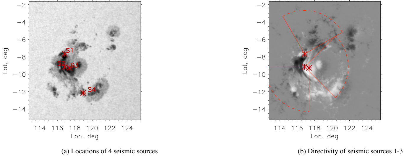
Fig. 5. (a) HMI white light image of the active region marked with the egression maps of the seismic sources 1-4; (b) Directivity maps of seismic sources 1-3 derived with directional holography shown by the sectors with detectable acoustic signals marked by the solid and dashed red lines.
