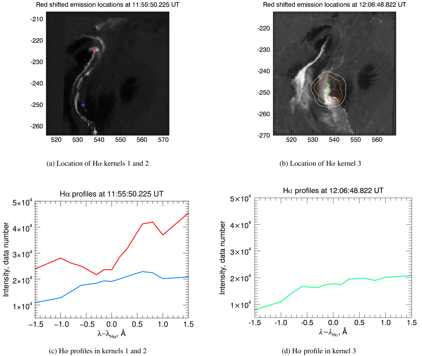
Fig. 14. Top plots: Red wing emission ( \lambda_{H\alpha} + 1.5 \text{ \AA} ) in the H\alpha line at 11:55:50 UT (flaring event 1) with the locations of (a) kernel 1 (seismic source 1) and kernel 2 (seismic source 2), shown by the red and blue circles, respectively, and the location of (b) kernel 3 (flaring event 2), marked by the green circle, observed at 12:06:48 UT. Bottom plots: (c) H\alpha line profiles in kernel 1 (red line) and kernel 2 (blue line) and (d) kernel 3 (green line) obtained with SST (arbitrary units) by taking the average over the pixels. The HXR contours obtained at 12:08:26 UT are over-plotted for the 25-50 keV channel with the contours at 0.25 of maximal intensity (white), 0.48 (light brown), 0.7 (medium brown), and 0.9 (dark brown).
