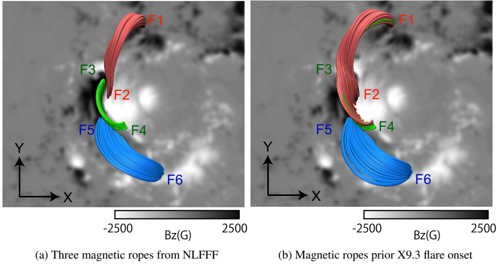
Fig. 1. Magnetic flux ropes formed during the X2.2 flare just prior to the 9.3 flare derived from NLFFF magnetic field reconstruction by Inoue et al. (2018) (a), which established the magnetic topology derived by the MHD simulations just prior to the X9.3 flare (b) with the loop footpoints being linked to the sunquake locations detected for this flare.
