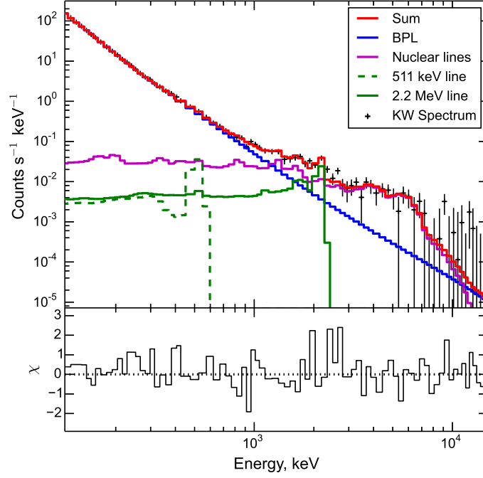
Fig. 3. Fitting of the time-integrated spectrum by the broken power law+NUCLEAR+511keV+2.2 MeV model (Lysenko et al. 2019). The component colour codes are given in the panel. The Konus/Wind (KW) data are shown using symbols, where the horizontal dashes indicate the energy range of each data point, while the vertical dashes indicate the corresponding statistical errors. The lower panel shows the fit residual. Adopted from Fig.3 of Lysenko et al. (2019).
