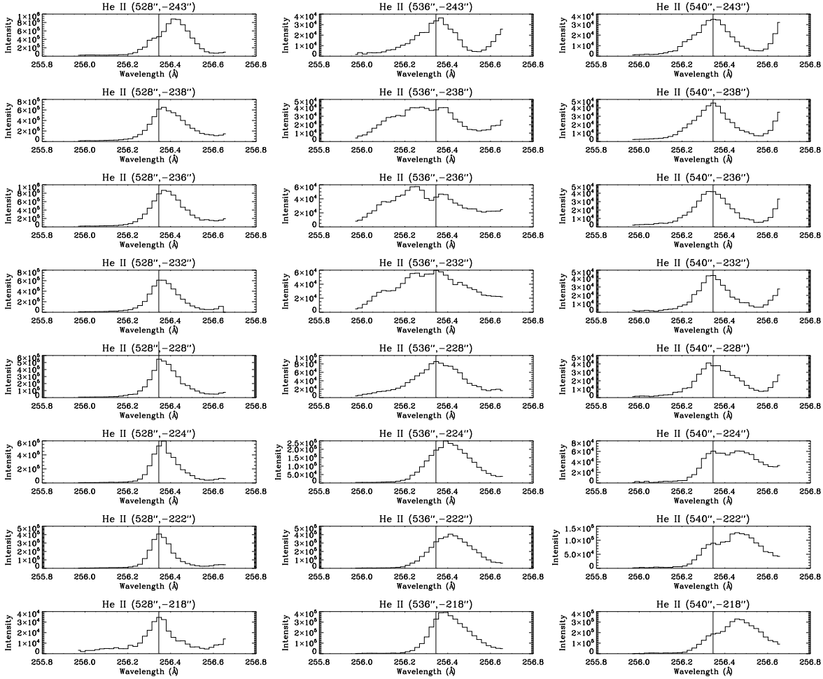
Fig. 10. Flaring event 1 (>11:55 UT): EIS He II line profiles from the selected locations at the slit positions associated with the locations of seismic sources (SQs) 1, 2, and 3. Heliocentric location is indicated above each profile. The vertical lines indicate the rest wavelength.
