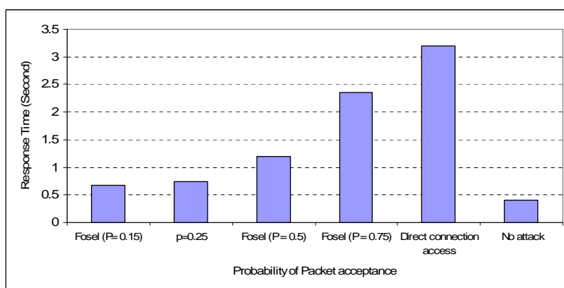
Figure 4.5: Average response time to download a file (size=671KB)
