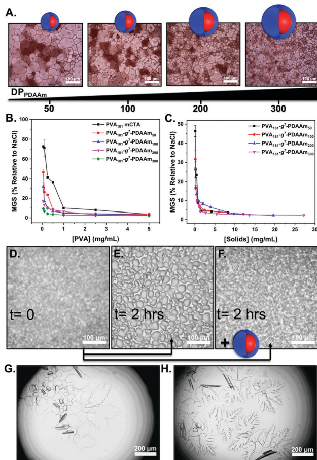
Fig. 3 Assessment of IRI and ice binding activity. (A) Cryomicrographs from the ‘split’ assay of nanoparticles. [PVA] = 0.05 \text{ mg mL}^{-1} ; (B) IRI activity correlated to [PVA]; (C) IRI activity in mass concentration; (D) ice growth in 45 wt% sucrose t = 0 ; (E) t = 2 hours. (F) t = 2 hours plus 1 \text{ mg mL}^{-1} of \text{PVA}_{181}\text{-g}^7\text{-PDAAm}_{300} nanoparticles; (G) ice shapping of sucrose solution alone; (H), 1 \text{ mg mL}^{-1} of \text{PVA}_{181}\text{-g}^7\text{-PDAAm}_{300} nanoparticles. MGS = mean grain size.
