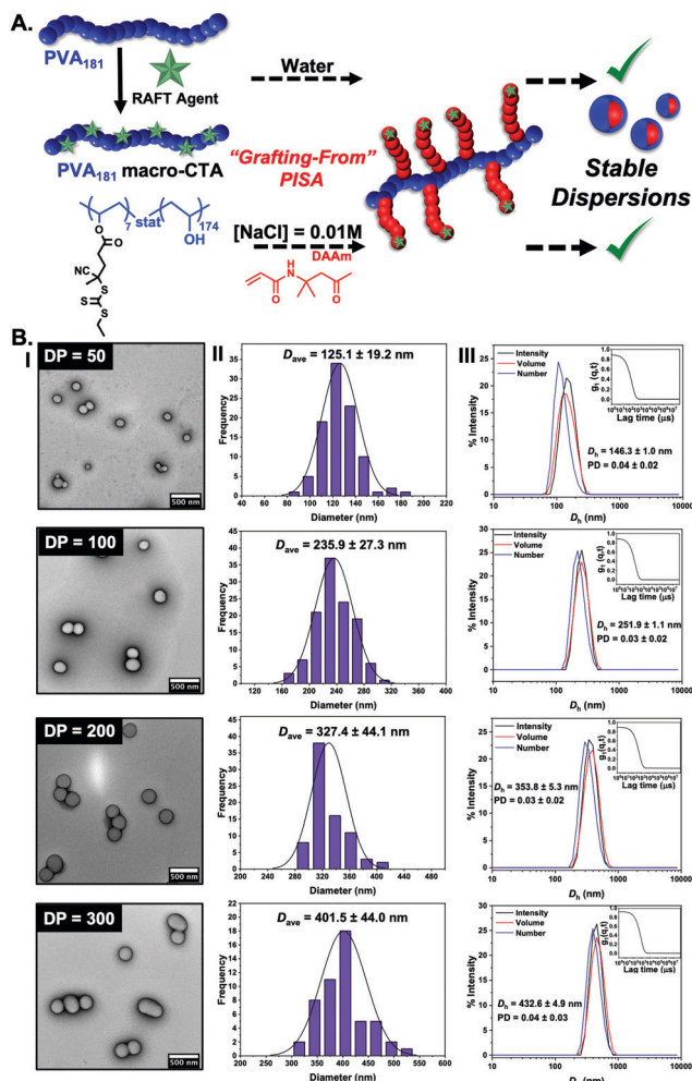
Fig. 2 (A) Schematic of the synthetic route employed for the preparation of \text{PVA}_{181}\text{-g}^7\text{-PDAAm}_n ( n = 50, 100, 200, 300 ) nano-objects at 10% w/w via thermally initiated RAFT dispersion PISA at 60 °C, using a \text{PVA}_{181} macro-CTA resulting in stable dispersion in both water and in saline; (B) characterisation of PDAAm-core nanoparticles as a function of PDAAm degree of polymerization by TEM (I), showing the particle size distribution (II) and also by DLS (III). See ESI† for cryo-TEM analysis. Histograms are from n > 50 , and DLS is averaged from n = 5 .
