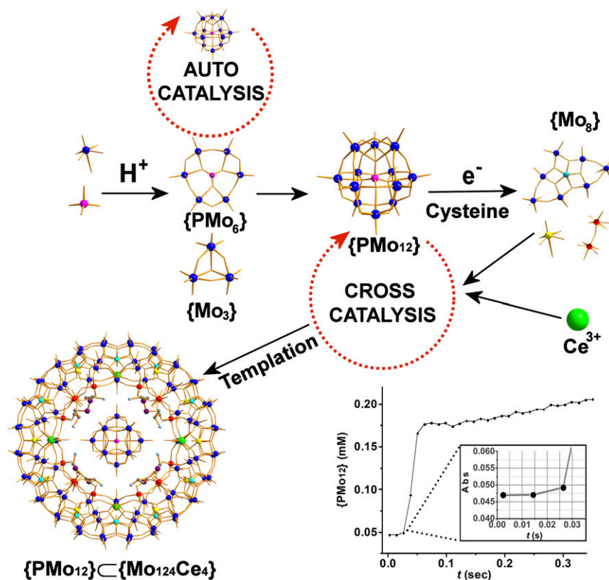
Fig. 5. Stochastic model predictions. Scheme of auto/cross-catalytic sequence for 1 . Scheme showing the templated assembly of the \{PMo_{12}\}C\{Mo_{124}Ce_4\} MB nanoring. Color scheme: \{Mo_1\} , yellow; \{Mo_2\} , red; \{Mo_3\} , blue (central MoO_7 pentagonal bipyramid, cyan); P, pink. The building blocks used in the formation of the Keggin species are postulated as \{Mo_3\} and \{PMo_6\} . Absorption vs. time profile of \{PMo_{12}\} (in H_2O at 24.3\text{ }^\circ C ), initial concentrations [Mo] = 0.7\text{ M} , [H^+] = 0.06\text{ M} . The circles are experimental data points. (Inset) The lag time observed at the early stages of the reaction.
