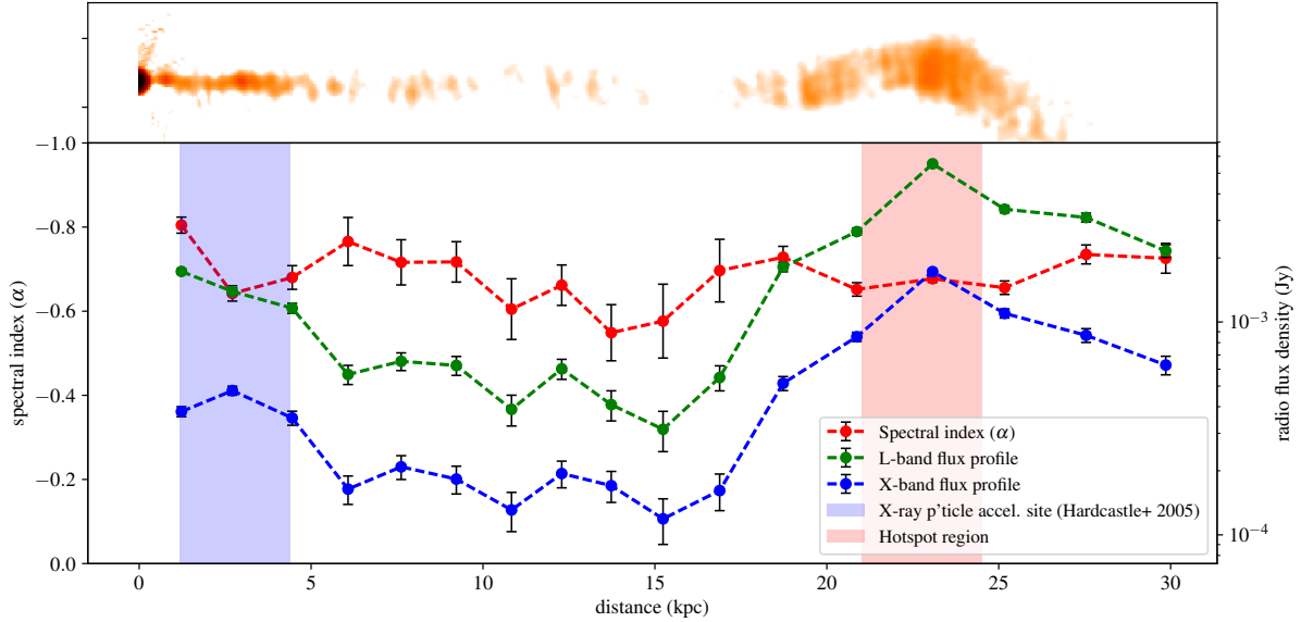
Figure 5. Profile of spectral index, \alpha along the NW jet axis as a function of projected distance from the galaxy central region. Also shown are the respective flux density distributions measured at 1.5 and 8.5 GHz at a resolution of 0.5-arcsec. Shown on the plot are also regions of X-ray enhancements, and so of rapid particle acceleration, as observed by Hardcastle et al. (2005) in a Chandra and XMM-Newton study of 3C 465 – colour coded in blue tone; and the NW hotspot region – colour coded in red tone. The top panel shows an \sim 45^\circ westward rotation of the NW jet used in our spectral analysis.
