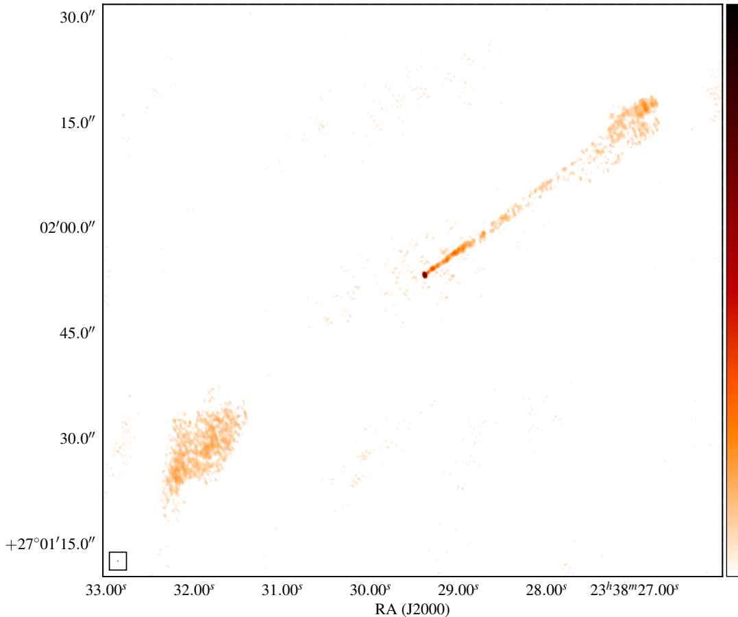
Figure 2. 0.27 \times 0.15 -arcsec resolution radio map of the WAT source 3C 465 observed at L-Band ( \sim 1.5 GHz) continuum frequencies with the e-MERLIN array – showing the sidedness of the radio jet (note the visible bright knotty structures at the jet base and the elliptical shape of the recovered primary beam)
