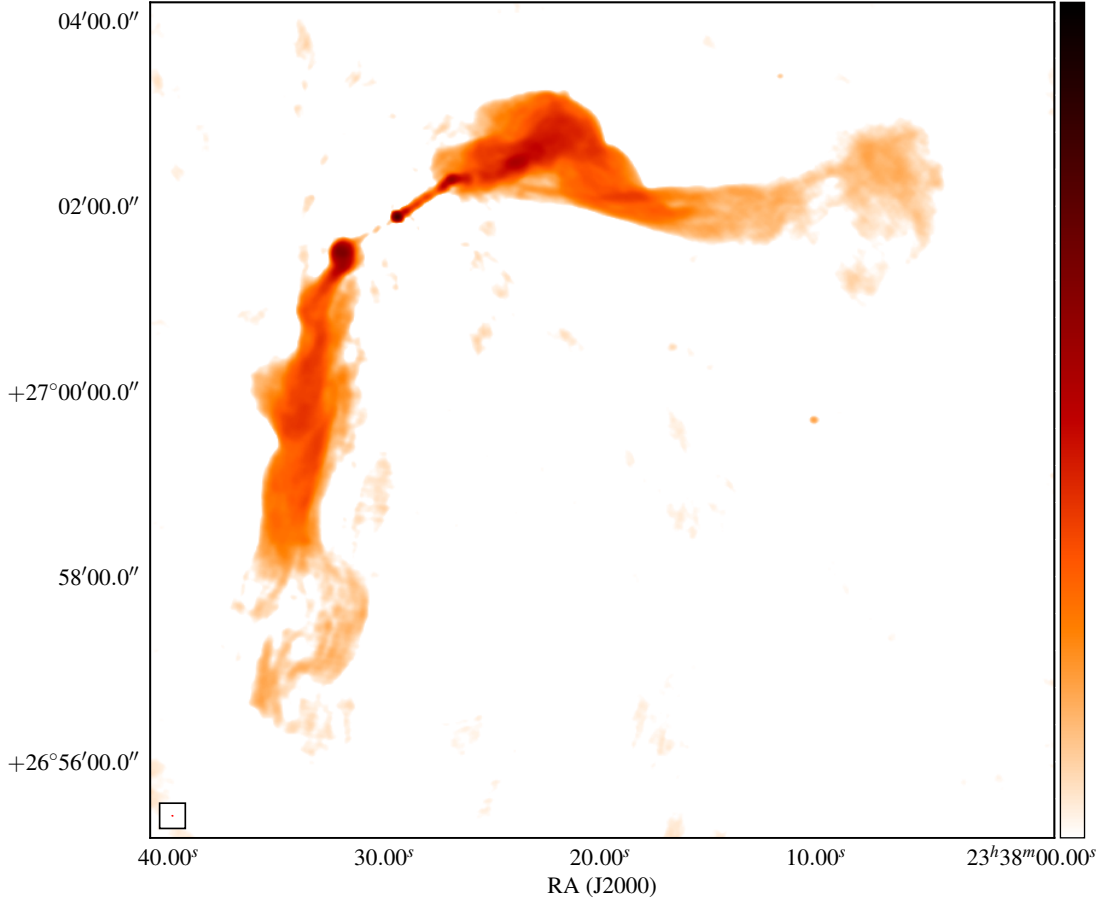
Figure 1. 1.37 \times 1.13 -arcsec resolution radio map of the WAT radio galaxy 3C 465 observed in A and B-configurations of the expanded VLA at L-Band ( \sim 1.5 GHz) continuum frequencies – showing the peaked central emission and the elongation of the overall radio structure in the NW-SE direction.
