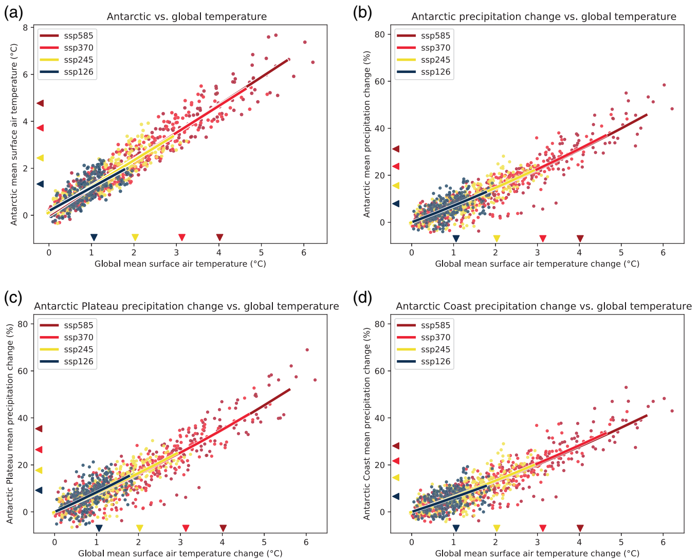
FIGURE 1 (a) Antarctic versus global mean SAT change for all available models (1st ensemble member) and four scenarios. Each dot is a 5-year average time-slice difference relative to the 1995–2014 mean. Regression lines are shown to quantify possible inter-scenario differences in GSAT-relative temperature projections. (b–d) Antarctic precipitation change against GSAT change (b), and separately also over the plateau ( h > 1,500 ) (c) and at coastal regions ( h < 1,500 m) (d). The regression lines in (b–d) are an exponential fit y = \exp(a \cdot T) - 1
