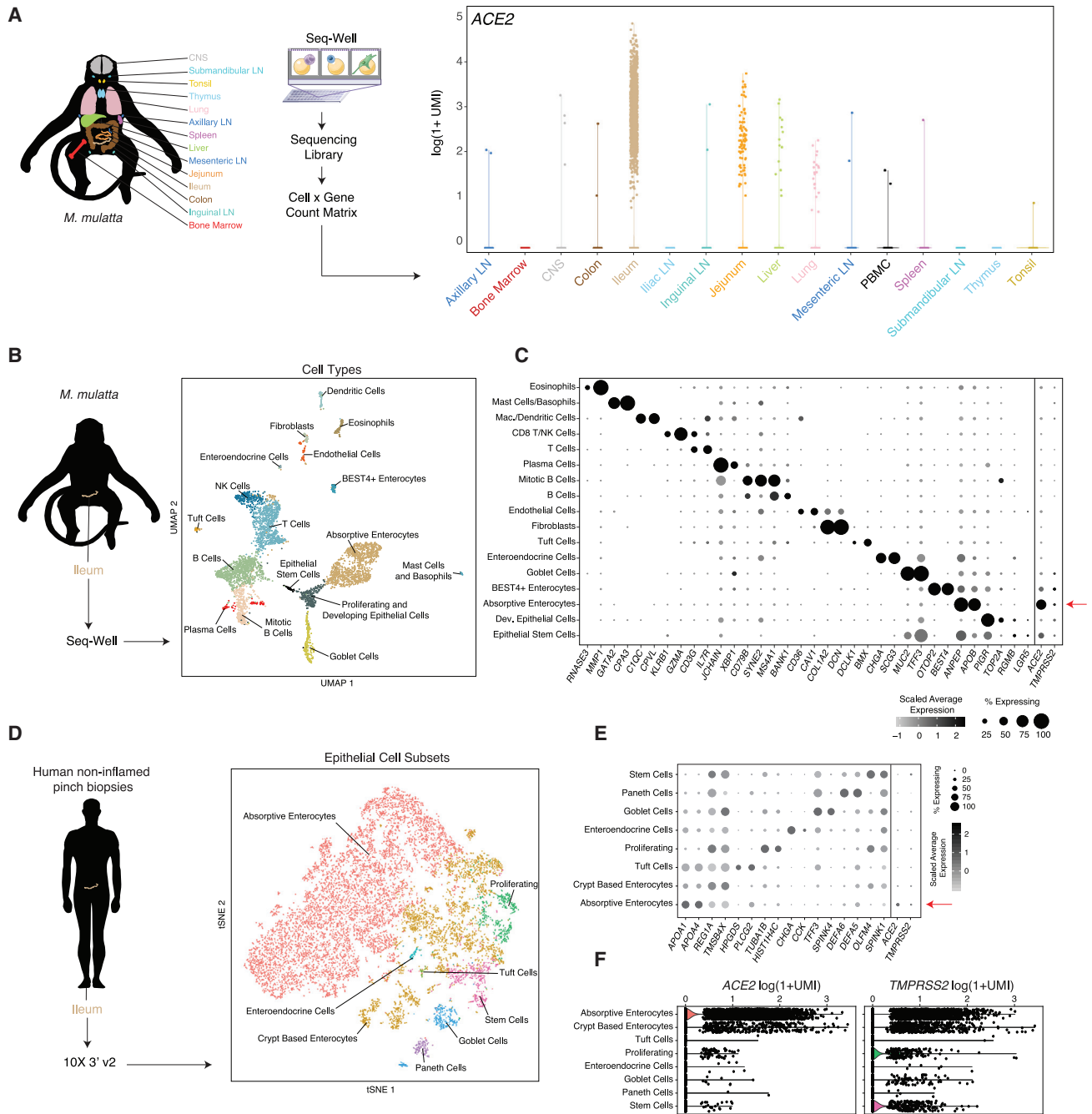
Figure 3. NHP and Human Ileal Absorptive Enterocytes Co-Express ACE2 and TMPRSS2
