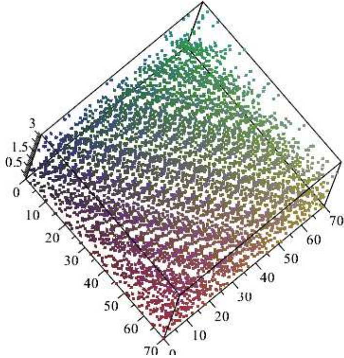
Figure 1: 3D plot of V_{k,l} against k, l for a travelling wave solution of the discrete KdV equation (3) given by V_{k,l} = v_{4k-3l+1000} where v_m satisfies (19) with N = 4 , M = 3 , \alpha = -1 and initial data v_j = 1 for 0 \leq j \leq 5 , v_6 = 3 .
