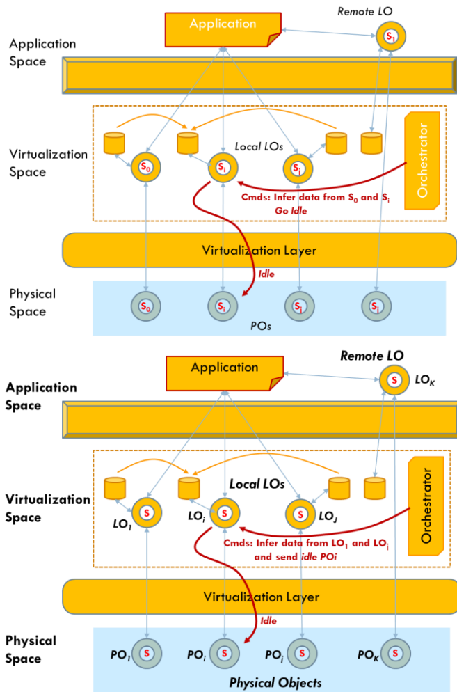
Figure 13 - Smart orchestration of Digital Twins
