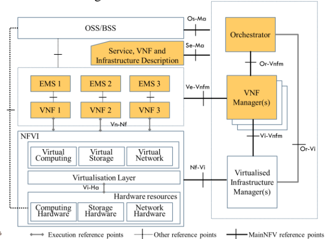
Figure 6 - ETSI architectural framework for Network Function Virtualization [111]
