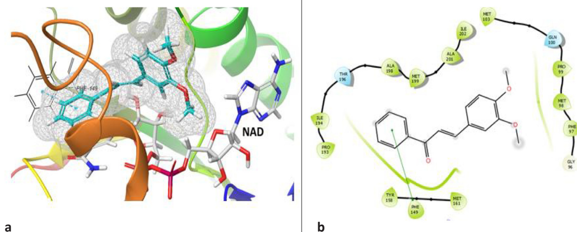
Fig. 6. (a) Shows the predicted interaction mode of compound 1a within the binding site of the InhA of Mycobacterium tuberculosis . InhA is shown as secondary structures with helices (green) and sheets (yellow). Compound 1a is shown in the teal capped stick format. Van der Waals surface around compound 1a is shown in mesh format. NAD is shown in element type format (Nitrogen in blue, Oxygen in red, Phosphorous in magenta). Pi-Pi stacking interaction is shown as teal dashed line between the phenyl rings of Phe 149 and the compound 1a . This image has been generated by using Schrodinger drug design software. (b) Shows the ligand interaction map of the compound 1a with the active site residues of the InhA. The proposed interaction mode of compound 1a is shown in the stick format. Pi-Pi stacking is shown in green line.
