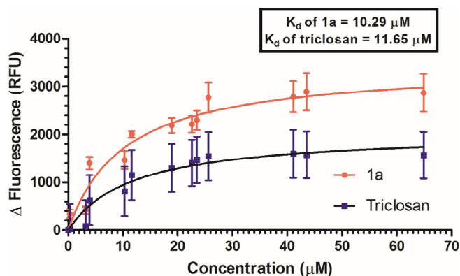
Fig. 5. Saturation binding assay using intrinsic tryptophan fluorescence to quantify association of increasing concentrations of ligands 1a and triclosan with InhA ( n = 3 ). The figure shows the K_d values (11.65 \mu\text{M} and 10.29 \mu\text{M} ) for triclosan and 1a . Data were fitted using GraphPad Prism, relative fluorescence units (RFU). The experiments were performed in biological replicates of n = 3 and the error bars represent the standard error bars of mean (SEM).
