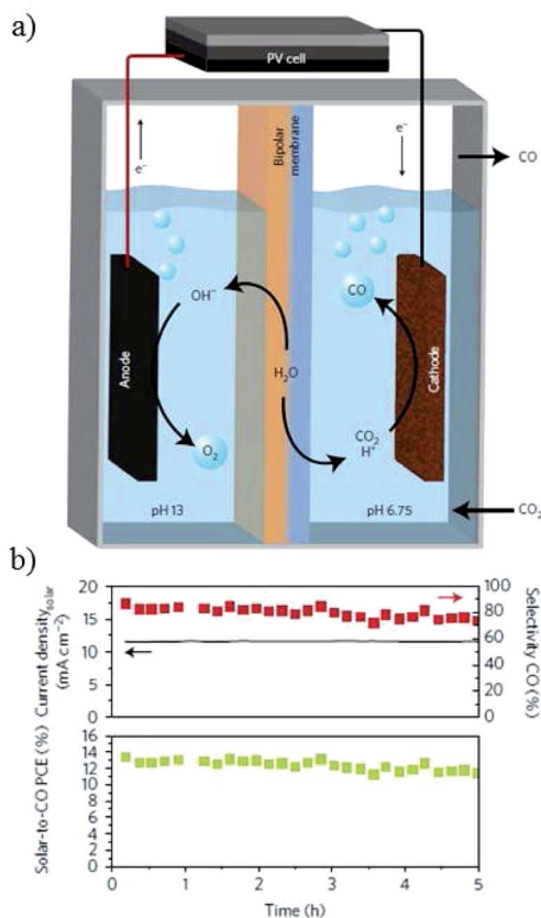
Fig. 33 (a) Schematic of PEC \text{CO}_2 reduction with PV cell. (b) Solar-to-CO conversion efficiency and selectivity of CO versus time. Experimental conditions: 0.1 M \text{CsHCO}_3||0.25\text{ M CsOH} , -0.55\text{ V vs. RHE} , PV cell (0.5625 \text{cm}^2 , 100 \text{mW cm}^{-2} , 2.38 V). Reproduced from ref. 61 with permission from Springer Nature, 2017.
