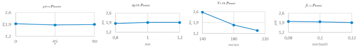
Fig 7. Main effect plot for Surface Roughness. Machine #2.
