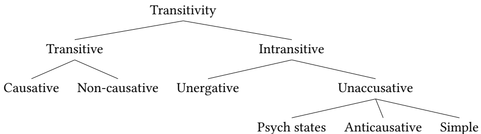
Figure 1: Subtypes of predicates as relevant for a typology of applicatives (Cuervo 2015b: 130)
