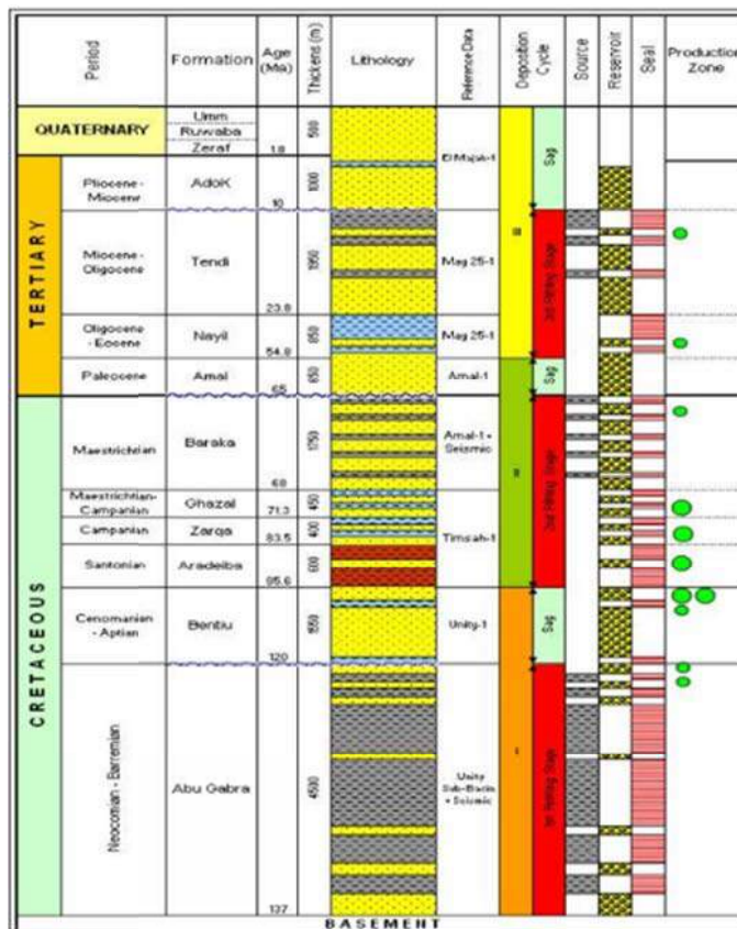
Figure 2: Stratigraphic units of the Muglad rift basin, SW Sudan, their lithology and depositional environment (adapted from Schull 1988).
