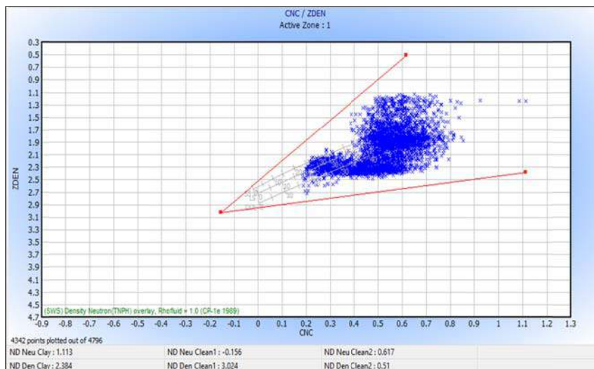
Figure 6: Lithology identification from density – neutron crossplot (Jake South -15).
