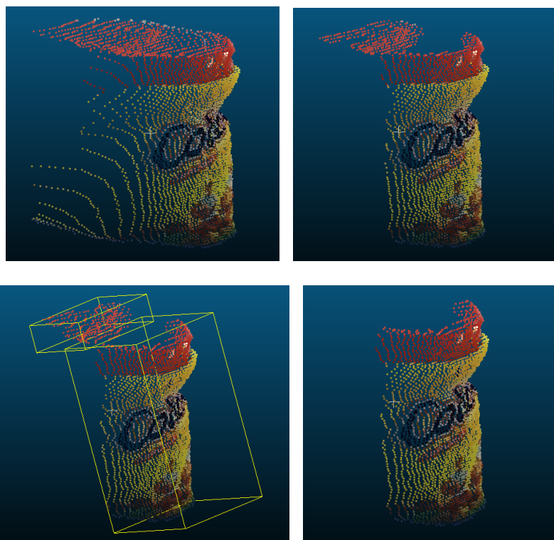
Figure A.8: Partial view with noise (top left), SOR/ROR filtered (top right), euclidean clusters detected (bottom left), keeping the biggest cluster (bottom right).
