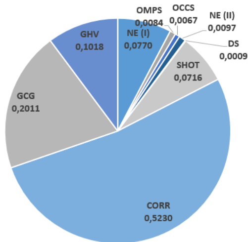
Figure 3.26: Phase time distribution using SHOT on Jetson TK1.
