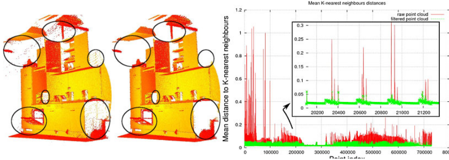
Figure A.6: Effects of the statistical outlier removal filter, original cloud (left) and filtered one (right). The plot shows the mean k -nearest neighbor distances in a point neighborhood before and after applying SOR filter (Figure reproduced from [88]).
