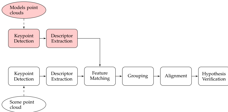
Figure 3.1: Object recognition pipeline implemented on the CPU. Red phases are performed offline while blank ones are live as the sensor provides information.
