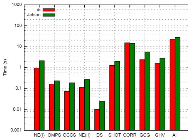
Figure 3.25: Mean execution times for all phases, Intel i5 vs Jetson TK1. Notice that the y-axis scale is logarithmic.
