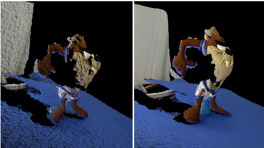
Figure 3.2: Raw point cloud of a scene with the Tasmanian model on it (left) and the same point cloud applying a bilateral filter with \sigma_s = 15.0f and \sigma_r = 0.05f (right). In this case, the filtering is excessive and it leads to information loss.
