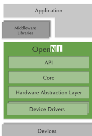
Figure 2.1: OpenNI 2.0 SDK Architecture.
