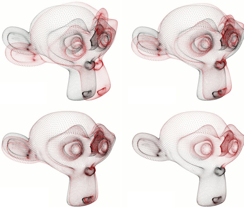
Figure 3.13: Cloud alignment refinement with ICP algorithm. The original point cloud in gray and the ICP aligned cloud in red. Initial positions (top left), four ICP iterations after (top right), eight ICP iterations after (bottom left) and twelve iterations after (bottom right). (Figure reproduced from Point-clouds.org ).
