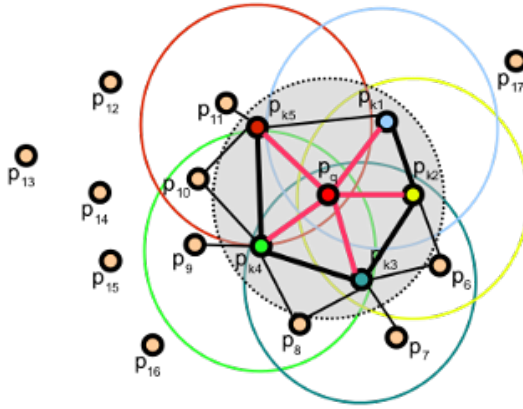
Figure 1.10: FPFH Neighbors of the current keypoint p_q in red linked by pink lines. For those points, each neighborhood is delimited by a colored circle. Bold lines represented relationships which are computed twice. (Figure reproduced from Pointclouds.org ).
