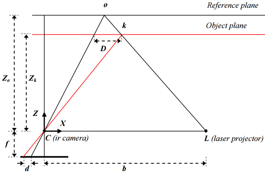
Figure 2.10: Kinect mathematical model (Figure reproduced from [58]).
