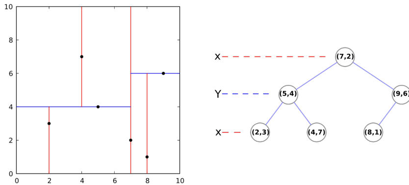
Figure 3.7: Example of a 2D k-d tree. (Figure reproduced from Wikipedia ).
