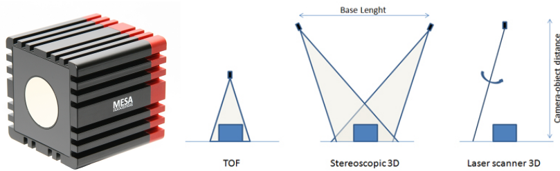
Figure 1.17: Left: SR4000 camera (Figure reproduced from SR4000 dataset [42]), Right: basic functioning schema of ToF , stereoscopic 3D and laser scanner systems (Figure reproduced from Robotshop.com ).
