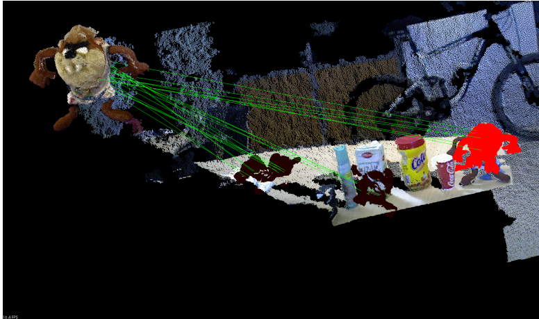
Figure 3.14: Recognition hypotheses verified with Global Hypothesis Verification; rejected false positive hypotheses in dark red, accepted true positive hypothesis in bright red. Green lines represent model-scene correspondences.
