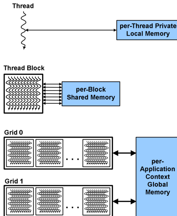
Figure 2.5: CUDA hierarchy of threads, blocks and grids with corresponding per-thread, per-block and per-application memory spaces.
