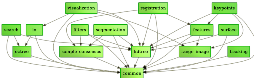
Figure 2.3: Point Cloud Library (PCL) dependency graph.
