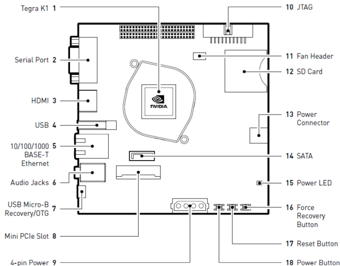
Figure 2.7: Jetson TK1 layout (Figure reproduced from [52]).
