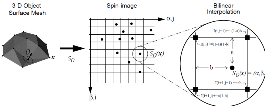
Figure 1.7: The addition of a point to the 2-D array representation of a spin-image. From left to right: projection, 2D array generation and contribution calculation with bilinear interpolation. (Figure reproduced from [32]).
