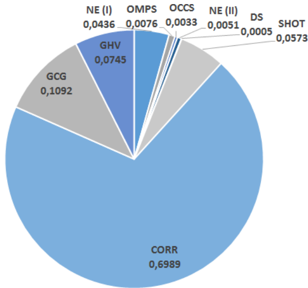
Figure 3.24: Mean execution times percentages for each phase using SHOT.
