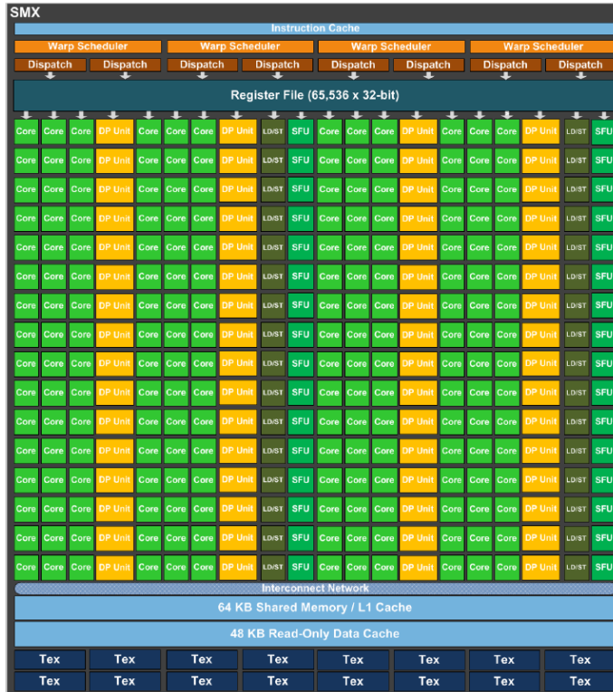
Figure 2.8: Block diagram of GK110 SMX, composed by 192 CUDA cores (single precision), 64 double precision units, 32 special function units and 32 load/store units. (Figure reproduced from the document Next Generation CUDA Compute Architecture: Kepler GK110 [55]).
