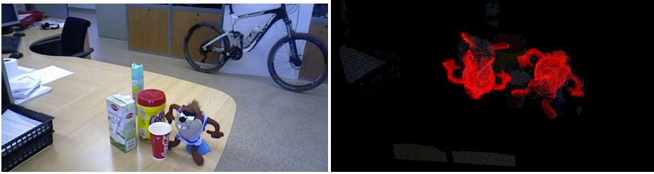
Figure 3.20: Validation scene (left) and recognition results with SHOT (right) one true positive (the recognized tasmanian model), one false positive (the wrongly recognized tasmanian in the milk) and seven true negatives.
