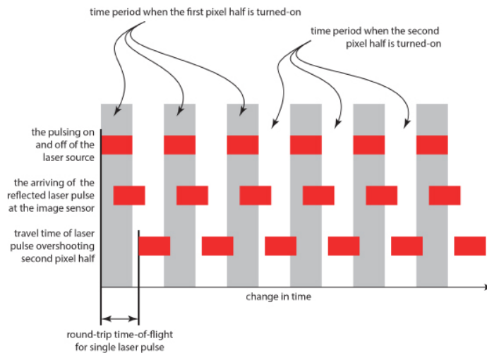
Figure 2.11: The indirect Time-of-Flight method (Figure reproduced from [60]).
