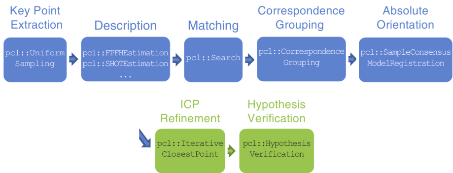
Figure 1.1: Local 3D recognition pipeline (Figure reproduced from [23]).
