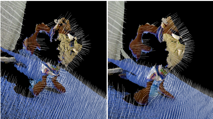
Figure 3.3: Normals of a raw point cloud of a scene with the Tasmanian model on it (left) and normals of the same point cloud applying a bilateral filter with \sigma_s = 15.0f and \sigma_r = 0.05f (right). The normals are much more stable thanks to noise reduction. It is necessary to find a balance between noise removal and geometric surface smoothing.
