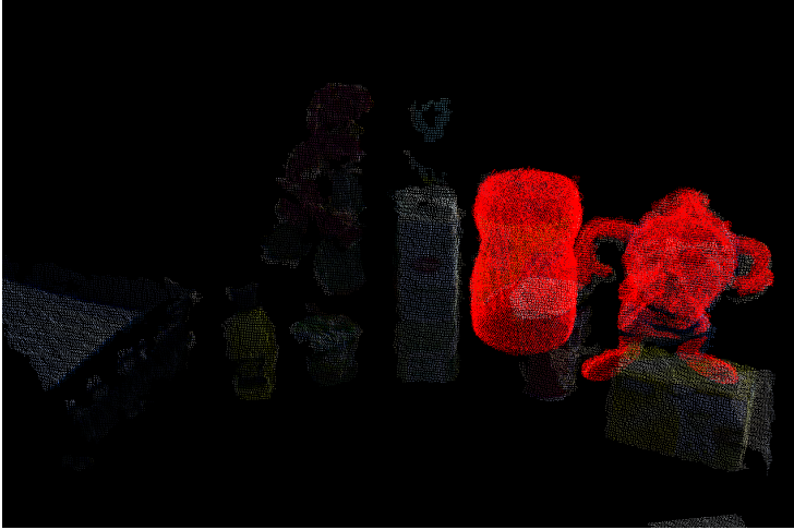
Figure 3.15: Global Hypotheses Verification example with multiple accepted hypotheses of different object models present in the scene.
