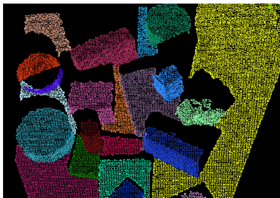
Figure A.7: Euclidean clusters extracted from a point cloud (Figure reproduced from Pointclouds.org ).
