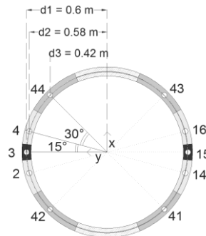
Figure 17. Plan view of the strain gauges position.
