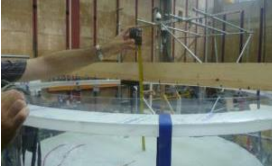
Figure 7. Measurement of grain settlements.
