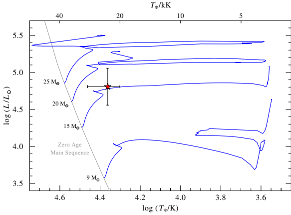
Fig. 7. Evolutionary tracks using the Geneva Stellar Models (Ekström et al. 2012) for solar metallicity and a rotation rate of v_{\text{ini}}/v_{\text{crit}} = 0.4 on ZAMS (it corresponds to 170 \text{ km s}^{-1} for an initial mass of 20 M_{\odot} ). Initial masses are: 9, 15, 20, and 25 M_{\odot} . The position of X1908+075 is marked by the red star.
