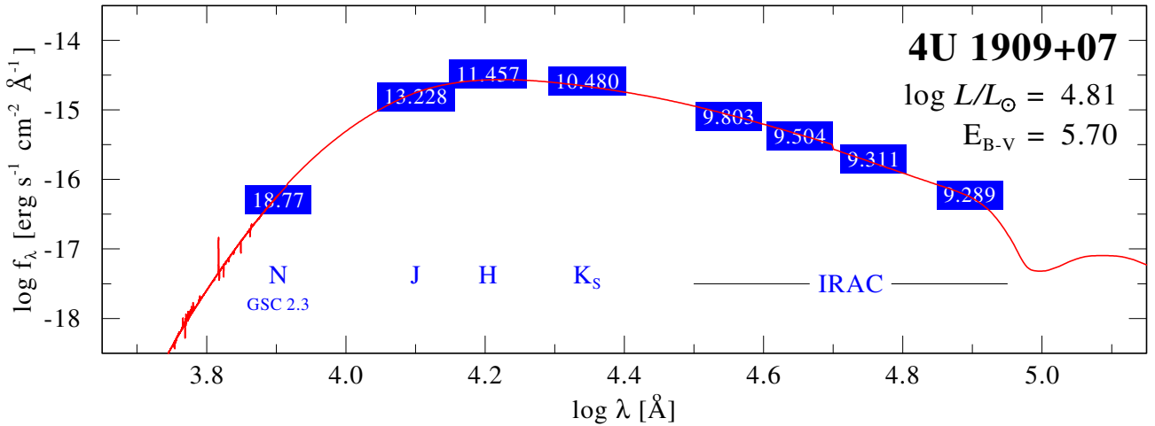
Fig. 3. Spectral energy distribution (SED) of the 4U 1909+07 donor star. The PoWR model (red solid line) is reddened such that it fits the observed photometry marks (blue boxes).
