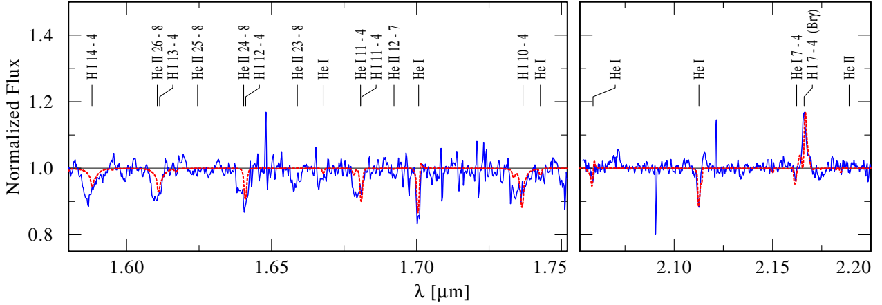
Fig. 5. Observed spectrum (thin blue line) – H band (left panel), K band (right panel) – compared with the best-fitting PoWR model (red thick dotted line). Noticeable spectral lines are identified.
