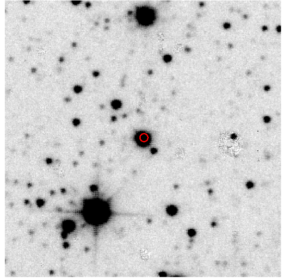
Fig. 1. UKIDSS image of the X1908+075 region. North is up and east is left. The red circle indicates the Chandra position of the X-ray source. Size of the image: 1' \times 1' .
