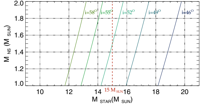
Fig. 6. Relations between the donor mass and neutron star mass. Lines of constant orbital inclination constructed from the mass function of Levine et al. (2004) are labelled. The X-axis range corresponds to the spectroscopic mass error margin, while the Y-axis range covers the range permitted for a neutron star mass (e.g. Lattimer 2012 ).
