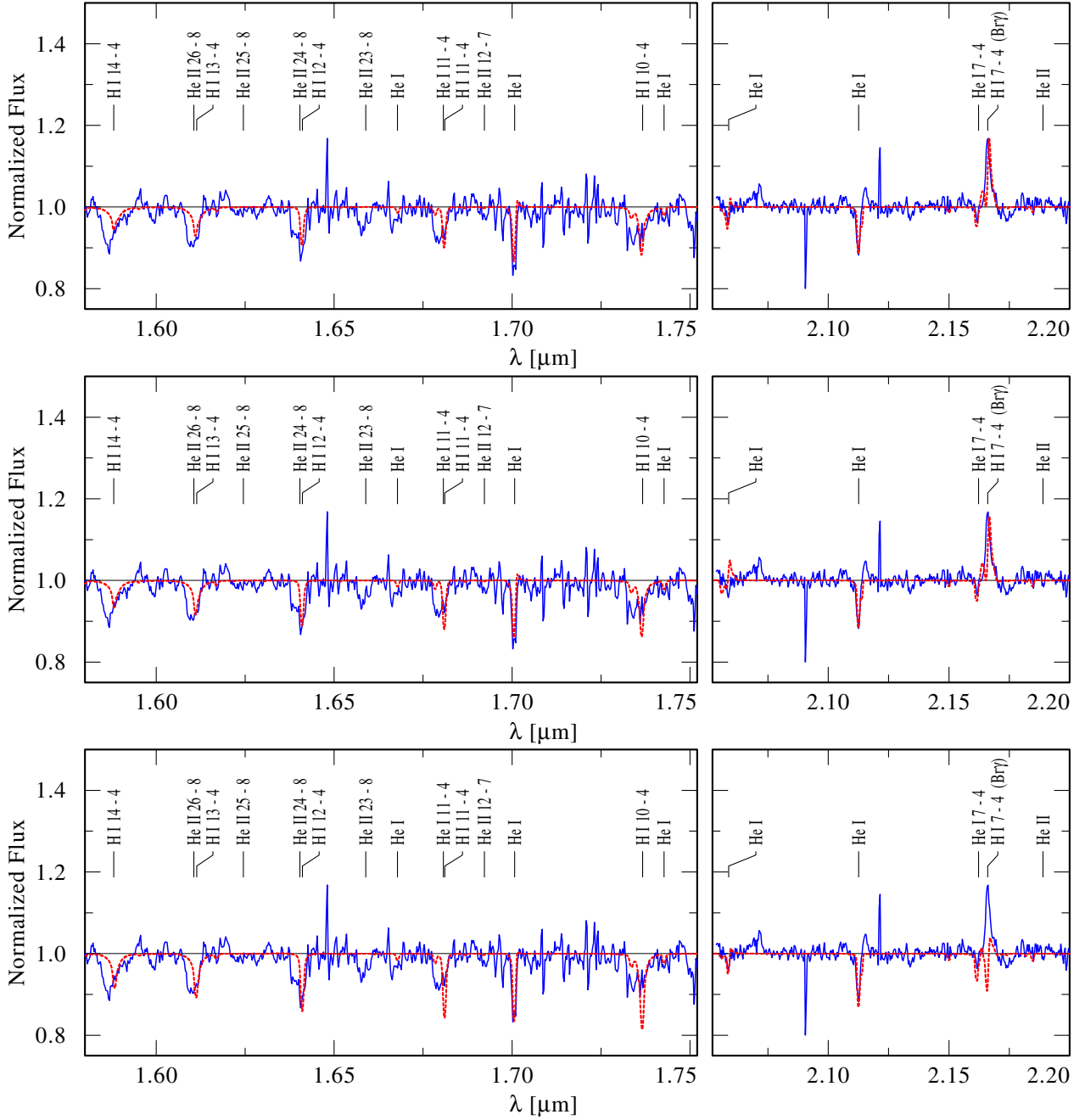
Fig. A.1. Observed spectrum (thin blue line) – H band (left panel), K band (right panel) – compared with the best-fitting PoWR model (dotted line) for different D factors: D = 10 (top panel); D = 4 (middle panel); D = 1 (low panel).
