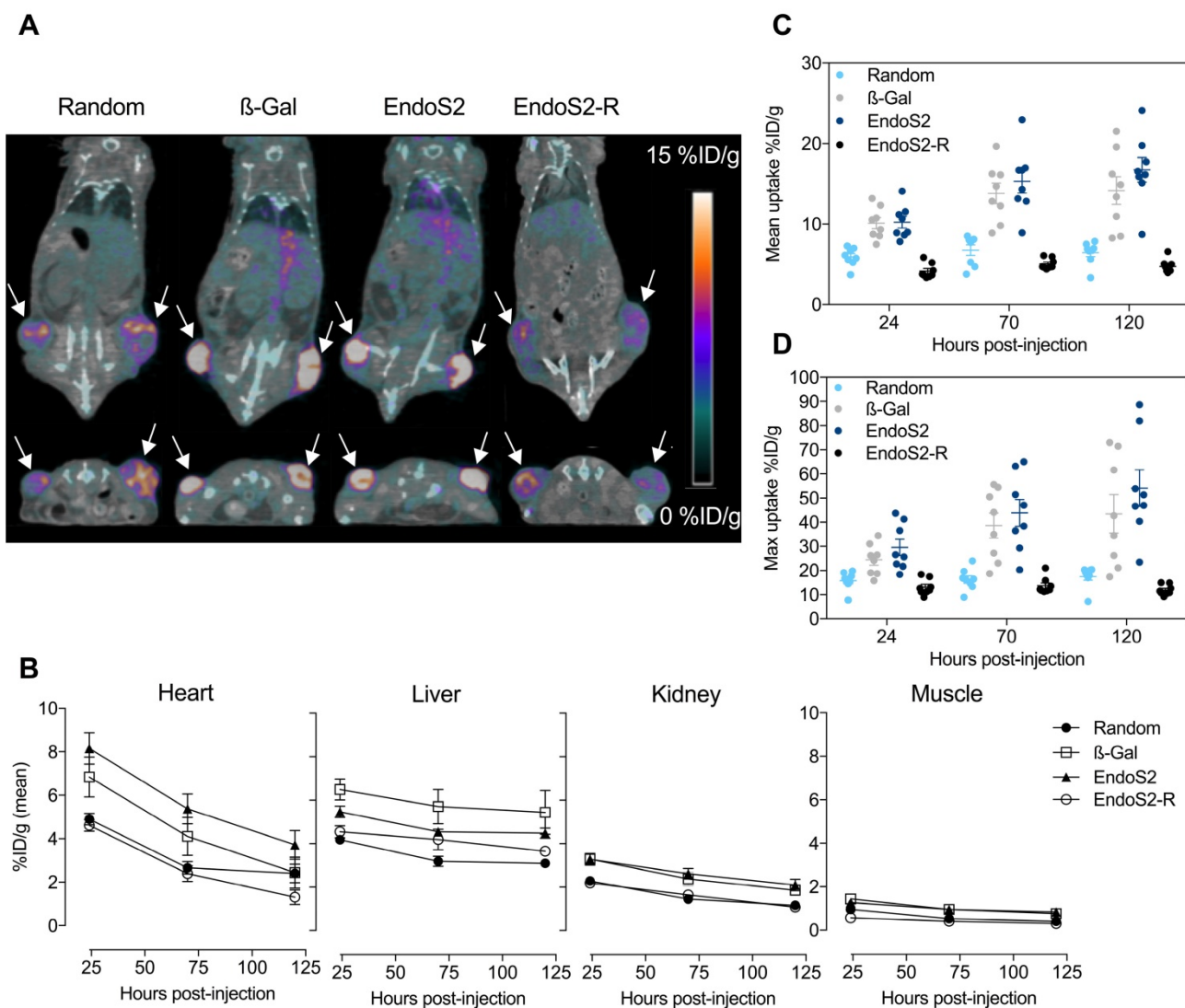
Figure 2: Longitudinal PET/CT imaging in SK-OV-3 xenograft bearing mice. (A) Representative coronal (top) and axial (bottom) images 70 hours post-injection of random, β-Gal, endoS2 and endoS2-R modified 89 Zr-DFO-trastuzumab. Arrows designate the tumors. (B) Image-derived biodistribution of 89 Zr-DFO-trastuzumab in major organs over the imaging time-course (N=4/tracer). (C) Mean and (D) maximum tumor uptakes at 24, 70 and 120 hours post-injection of tracers (N=4/tracer).
