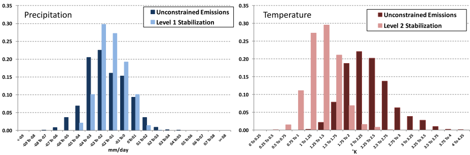
Fig. 2 Hybrid frequency distributions (HFDs) obtained from the IGSM simulations of changes in decadal-average seasonal precipitation for September–November (left panel) and decadal-averaged seasonal surface-air temperature change for December–February (right panel). Decadal average changes are taken as average of 2040s minus average of 1990s. The changes represent area-averaged values for the Zambezi River basin. Results are shown for an unconstrained (darker shaded bars) and the level 1 stabilization scenario (lighter shaded bars) ensemble simulations with the IGSM. Ordinate values indicate the fraction of the ensemble members that are contained within the binned seasonal precipitation and temperature changes
