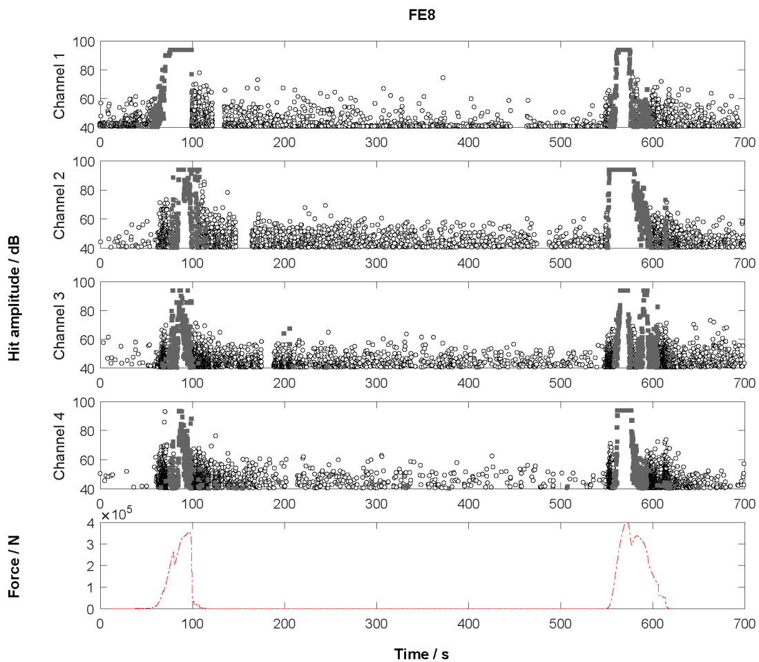
Figure 2: acoustic emissions (top four plots, showing amplitude of hits on channels 1-4) and force (bottom plot) against time for the compression experiment described above. Loading occurred in two separate phases. Square markers indicate hits where no transient was recorded: typically these are associated with periods of intense AE, and we attribute them to saturation in the electronics.
