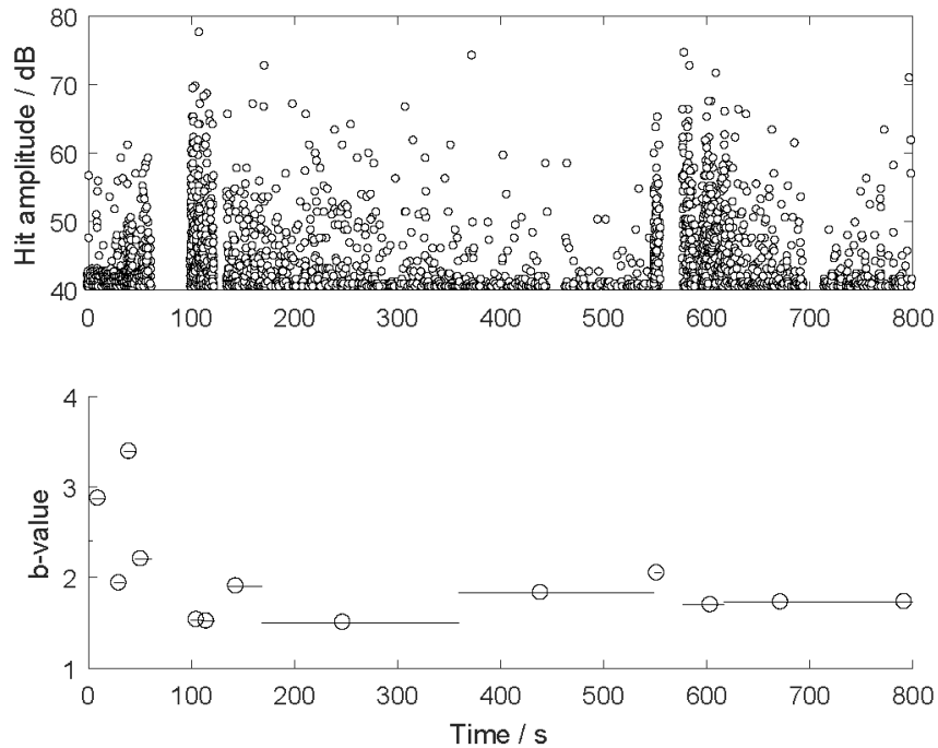
Figure 9: b-value variation (during the compression experiment, on channel 1) as a function of time (lower plot: the upper plot repeats the hit intensity data from figure 2, channel 1.) We select channel 1 as the only channel with > 5,000 data points. Each marker in the lower plot shows the b-value calculated for groups of ~1000 data points (sometimes adjusted to fit around breaks in the data). The horizontal lines show the temporal range of these groups of data points. b-values are relatively high at the start of the experiment, and on resumption of loading (around 550s).
