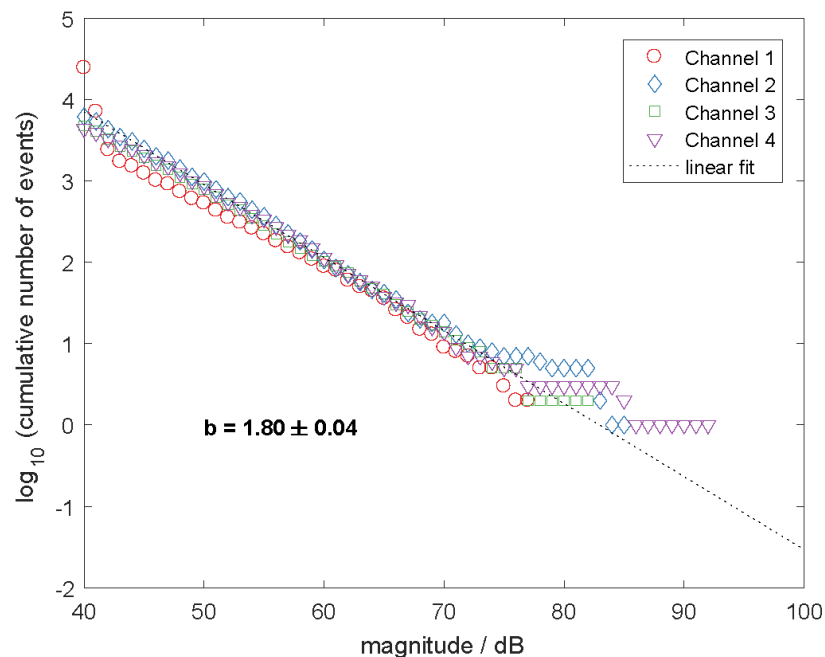
Figure 7: cumulative magnitude distribution for the AE hits from the compression experiment shown above (the data cover the entire duration of the experiment). The best-fit straight line is matched to the data from channel 2, up to 70dB magnitude, and has a slope b = 1.80 .
