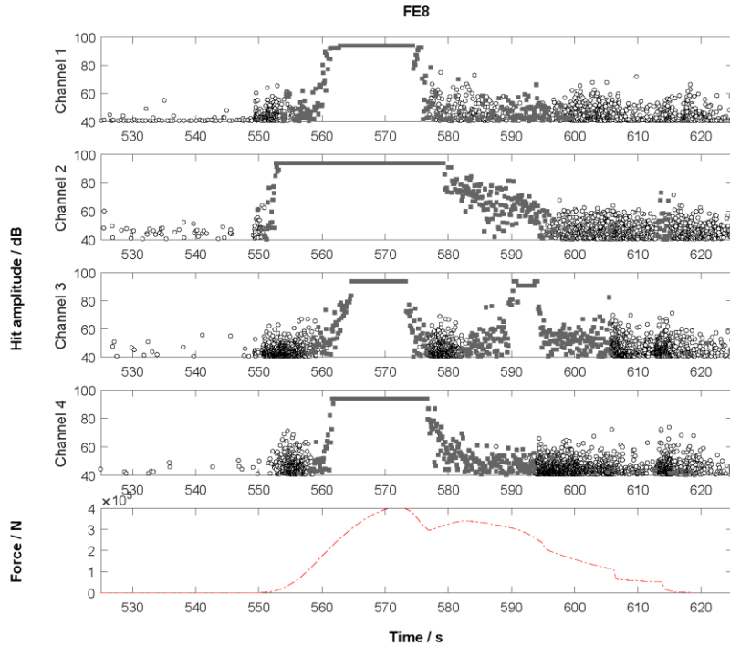
Figure 4: acoustic emissions and force against time for the compression experiment shown above, focussing on the second period of loading, from 525-625s.
