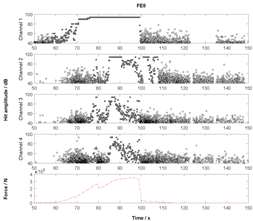
Figure 3: acoustic emissions and force against time for the compression experiment shown above, focussing on the first period of loading, from 50-150s.
