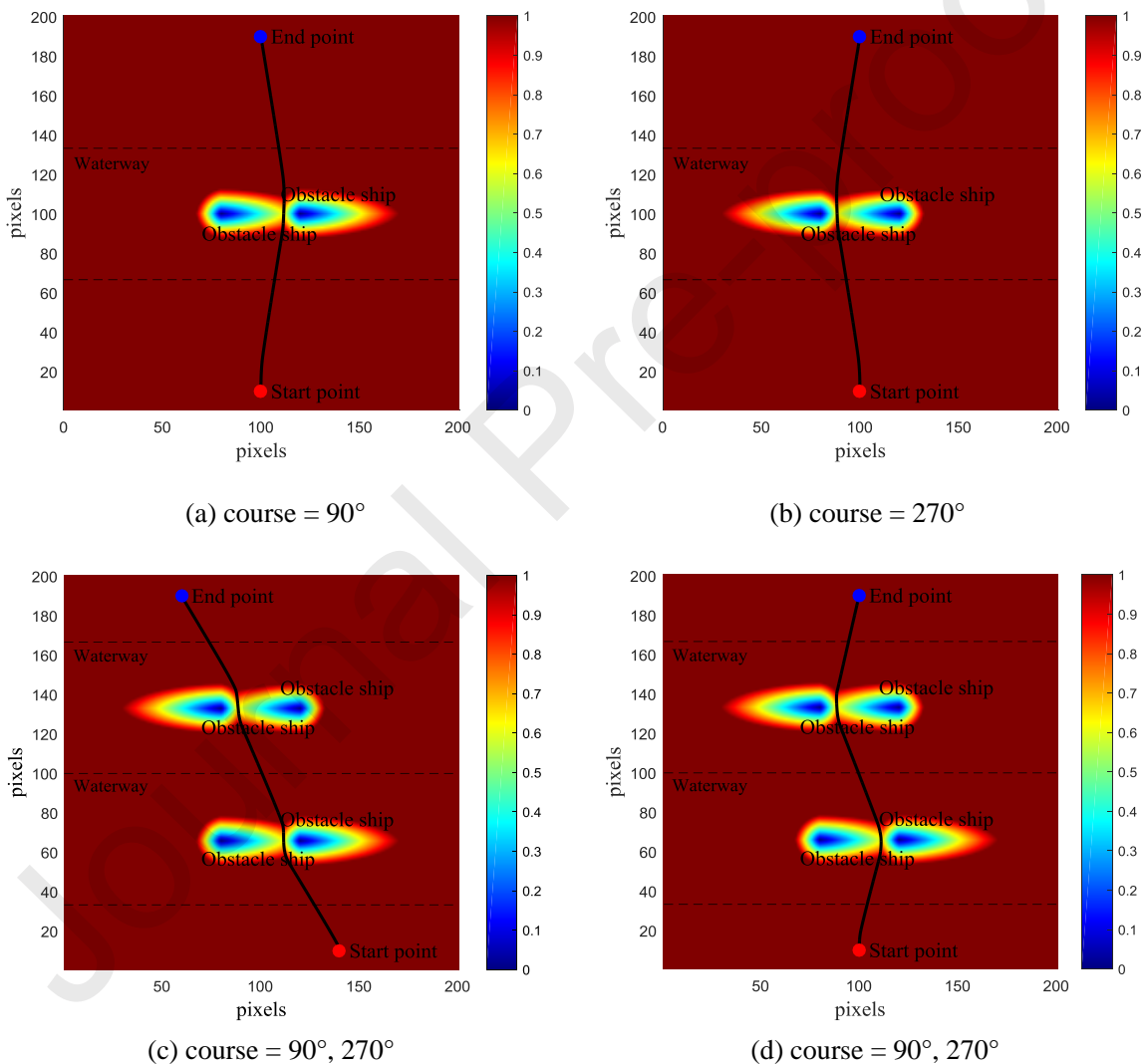
Fig. 7 The path planning result in complex environments with multiple dynamic obstacles.
