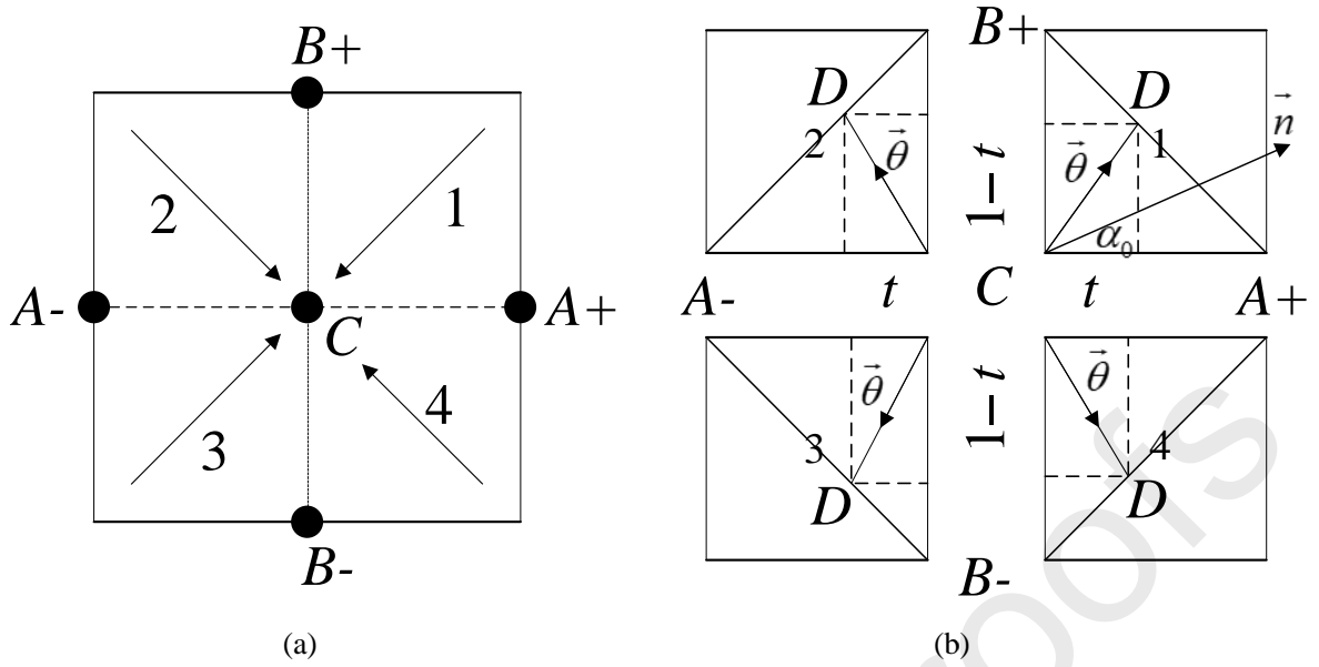
Fig. 1 The arrival time of point C is to be computed from one of the four quadrants around it. (b) The situations in four quadrants.
