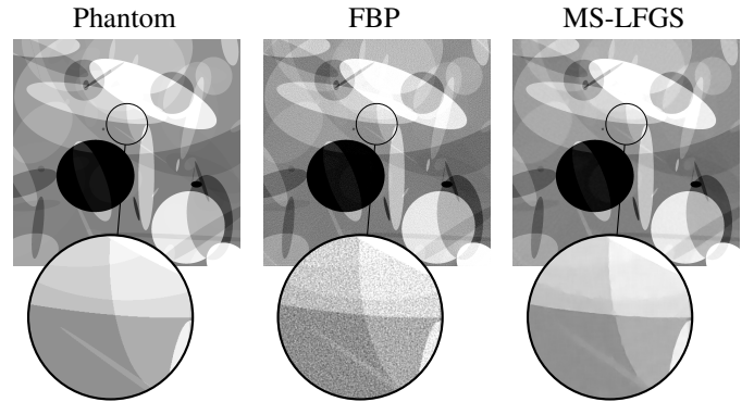
Fig. 5: Reconstruction of an ellipse phantom of size 1536^2 from 512 angles with 5% normally distributed random noise. (Left) Phantom used to create the data, (Middle) reconstruction by filtered backprojection, (Right) obtained reconstruction with MS-LFGS.
