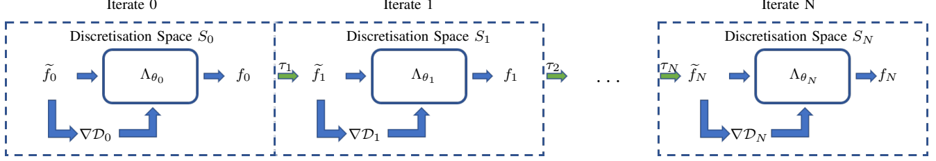
Fig. 1: Visualisation of the multi-scale learned gradient scheme (MS-LGS) as outlined in Algorithm algorithm 1. Each iteration is performed on their respective discretisation space, where the gradient \nabla \mathcal{D}_i := \nabla \mathcal{D}_i(f_i; g) is computed and the update is performed by the network \Lambda_{\theta_i} . After each update an upsampling by \tau_i to the next finer space is performed until the final resolution S_N is achieved.
