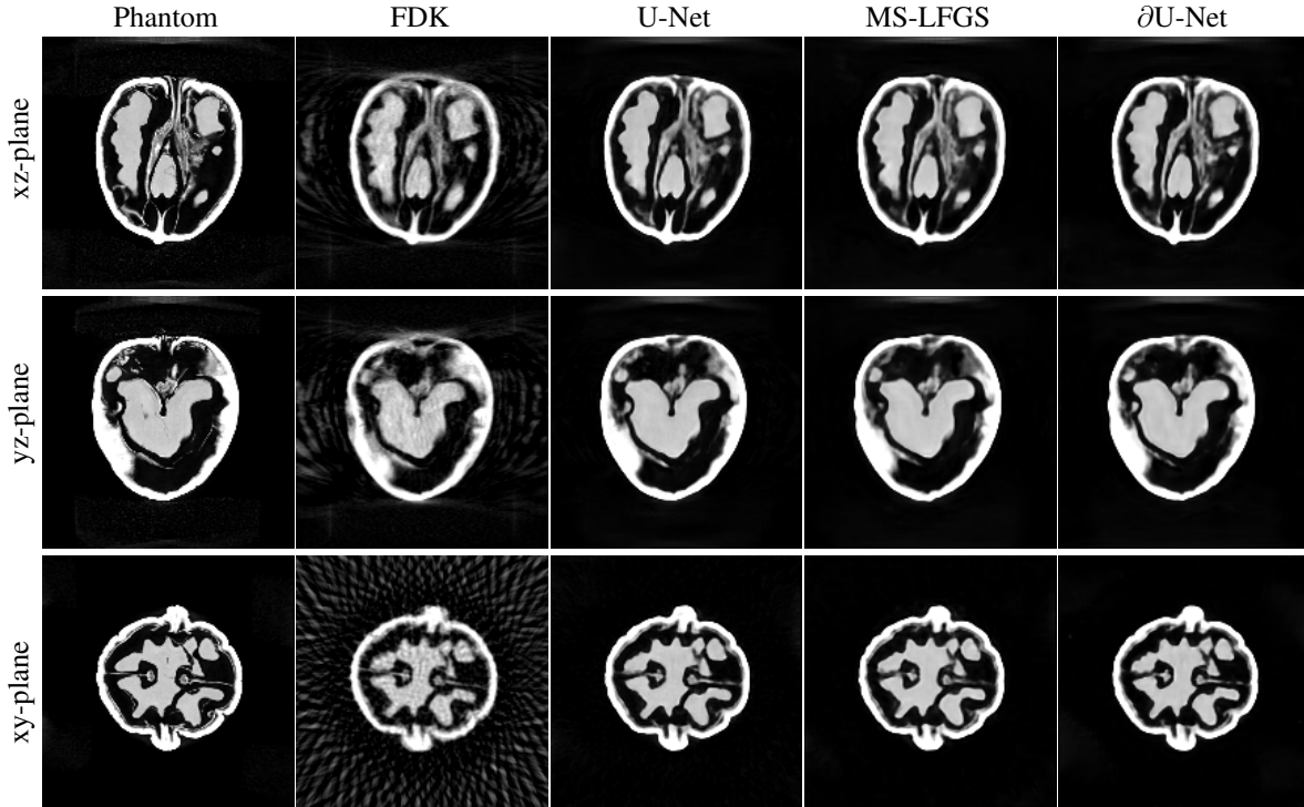
Fig. 3: Reconstructions of the Walnut used for testing from 60 angles. Reconstructions are compared to the phantom computed from a total of 1200 angles and three scanning positions to negate cone beam artefacts. The reconstruction by FDK is computed with Hann filter and frequency scaling h = 0.6 (PSNR=26.95). The proposed algorithm \partial U-Net (PSNR=34.69) is compared to post-processing by U-Net (PSNR=34.62) and the multi-scale approach MS-LFGS (PSNR=34.13) using a mini U-Net in each scale.
