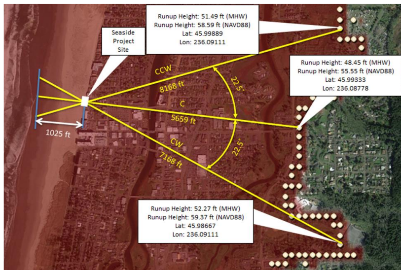
Figure 6. Energy Grade Line Analysis at building site in Seaside (McKamey & Robertson, 2019).
