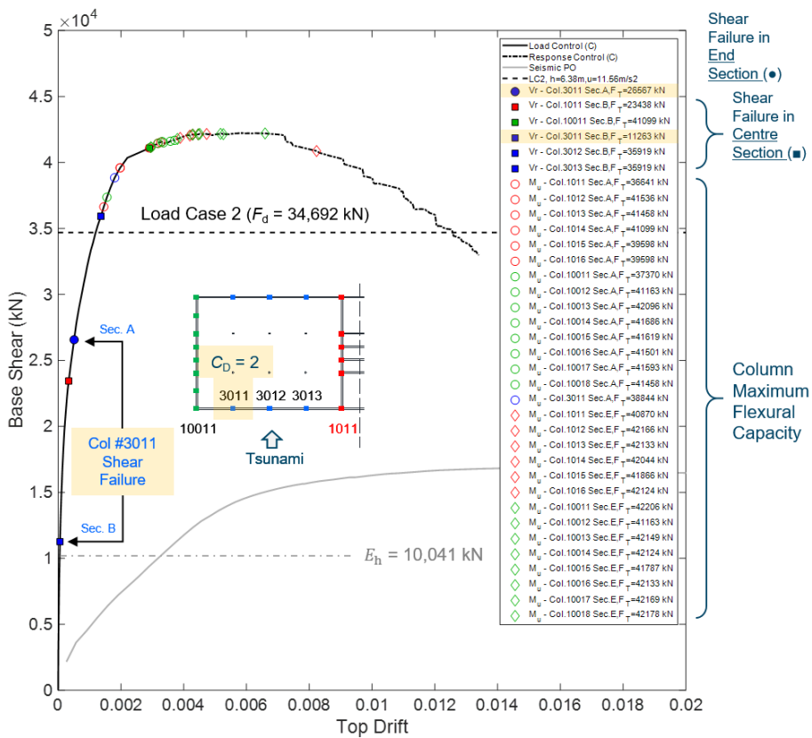
Figure 8: Base-shear-top drift curves from seismic PO and tsunami PO with load discretisation method S (top) and C (bottom), with sequence of maximum flexural capacity and shear failure attainment (for ground floor columns)
