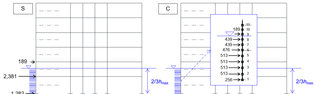
Figure 4: Loading discretisation methods S (left) and C (right).
