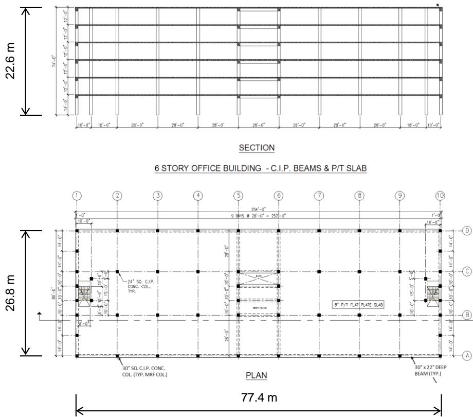
Figure 5. Prototype building (McKamey & Robertson, 2019).
