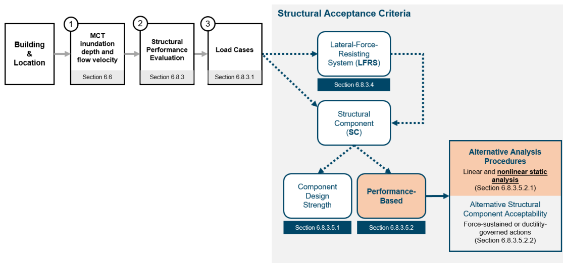
Figure 1. Tsunami nonlinear static analysis within the framework of ASCE 7-16 tsunami design provisions.
