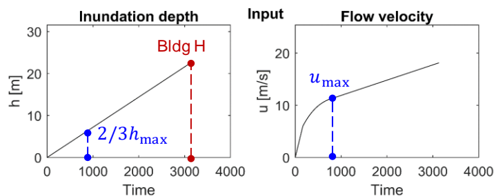
Figure 3: Inundation depth and flow velocity time histories for Phase 1.
