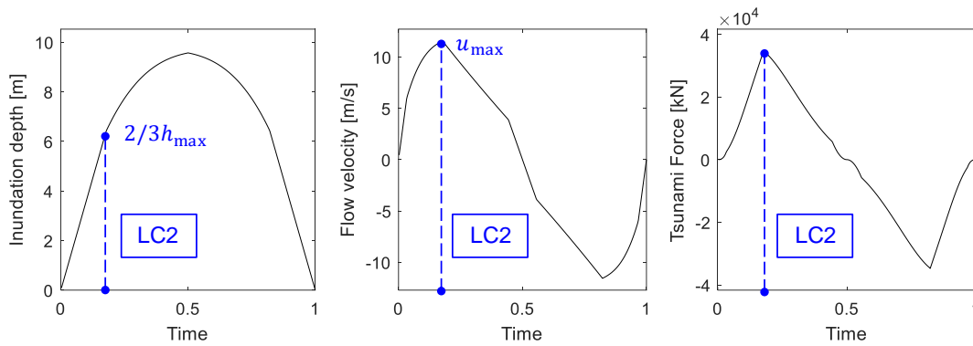
Figure 2: Tsunami inundation depth, flow velocity and force time-history curves at the building site in Seaside.
