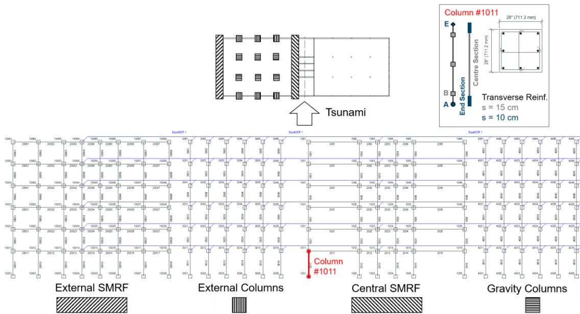
Figure 7: View of the two-dimensional finite element model (half of full prototype building).
