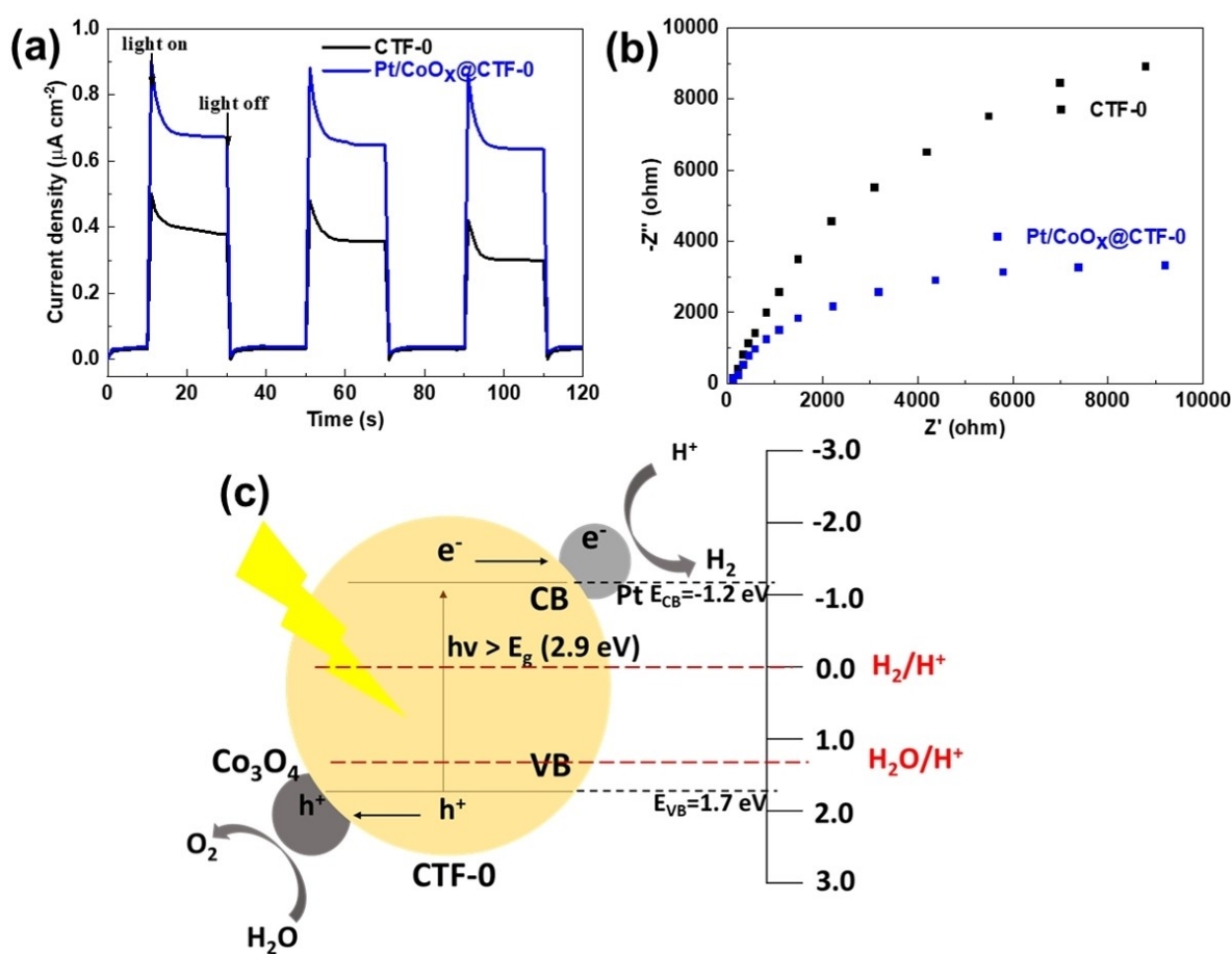
Figure 3. (a) transient photocurrent response, (b) electrochemical impedance spectroscopy Nyquist plots of CTF-0 and Pt/Co 3 O 4 @CTF-0 in 0.1 M Na 2 SO 4 with 0.4 V bias versus Ag/AgCl and pH=6.5, and (c) proposed schematic of the photocatalytic overall water splitting reaction mechanism on Pt/Co 3 O 4 @CTF-0.
