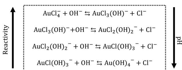
Fig. 2 Speciation reactions involving \text{AuCl}_4^- in water. As the pH increases, the degree of hydroxylation of the Au precursor increases. The higher is the degree of hydroxylation, the less reactive is the precursor.
