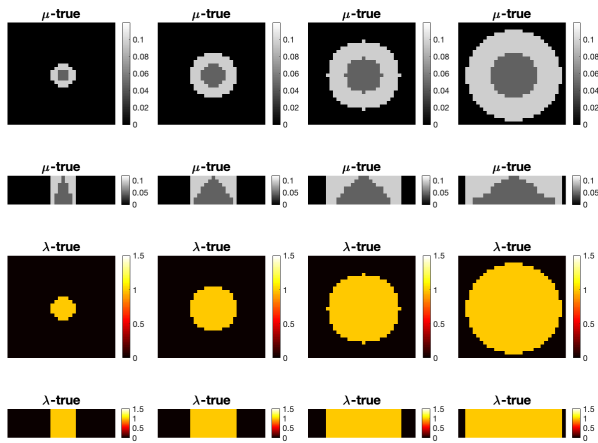
Fig. 1. Cylindrical Phantoms of increasing diameters: 8 cm (first column), 16 cm (second column), 24 cm (third column), 32 cm (fourth column). First and second rows: attenuation image axial and sagittal view. Third and fourth rows: activity image, axial and sagittal view. The attenuation is expressed in \text{cm}^{-1} , the activity is in arbitrary units.
