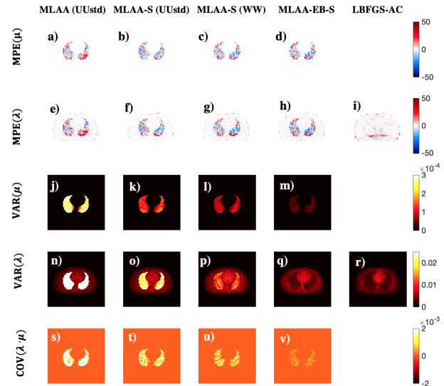
Fig. 6. Error metrics in the XCAT images for different reconstruction algorithms: MLAA (U std ), first column; MLAA-S (U std ), second column; MLAA-S (WW), third column; MLAA-EB-S, fourth column; LBFSGS-AC, fifth column. From the top to the bottom: MPE images [%] (a-d) and variance (VAR) (j-m) for the attenuation from 100 noise realisations; MPE images [%] (e-i) and variance (VAR) (n-r) for the activity image. Covariance (COV) images (s-v).
