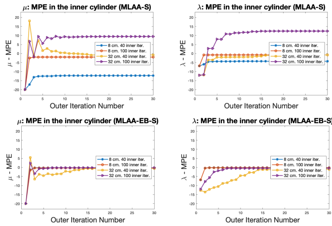
Fig. 5. MPE over outer iterations for the attenuation (left) and activity (right) estimations. First row: MLAA-S. Second row: MLAA-EB-S.
