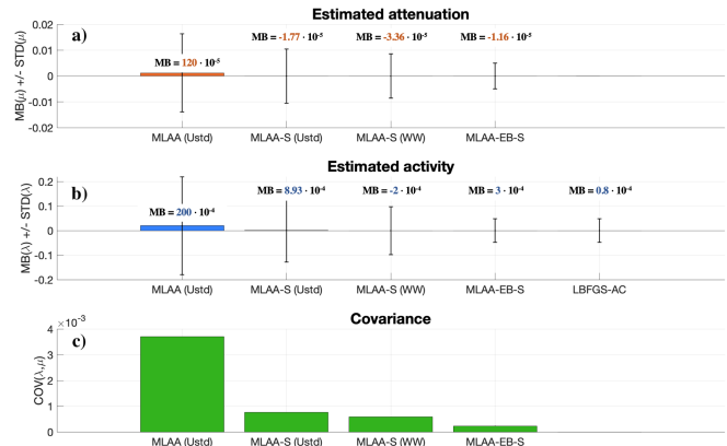
Fig. 7. Mean bias (MB) and standard deviation (STD), indicated as error bars, in the estimated attenuation (a) and activity (b); covariance (c). Obtained with: MLAA (U std ), MLAA-S (U std ), MLAA-S (WW), MLAA-EB-S and LBFSGS-AC. All mean values are computed over the lung ROI. \hat{\lambda}^{\text{true}} = 0.3260 and \hat{\mu}^{\text{true}} = 0.02865
