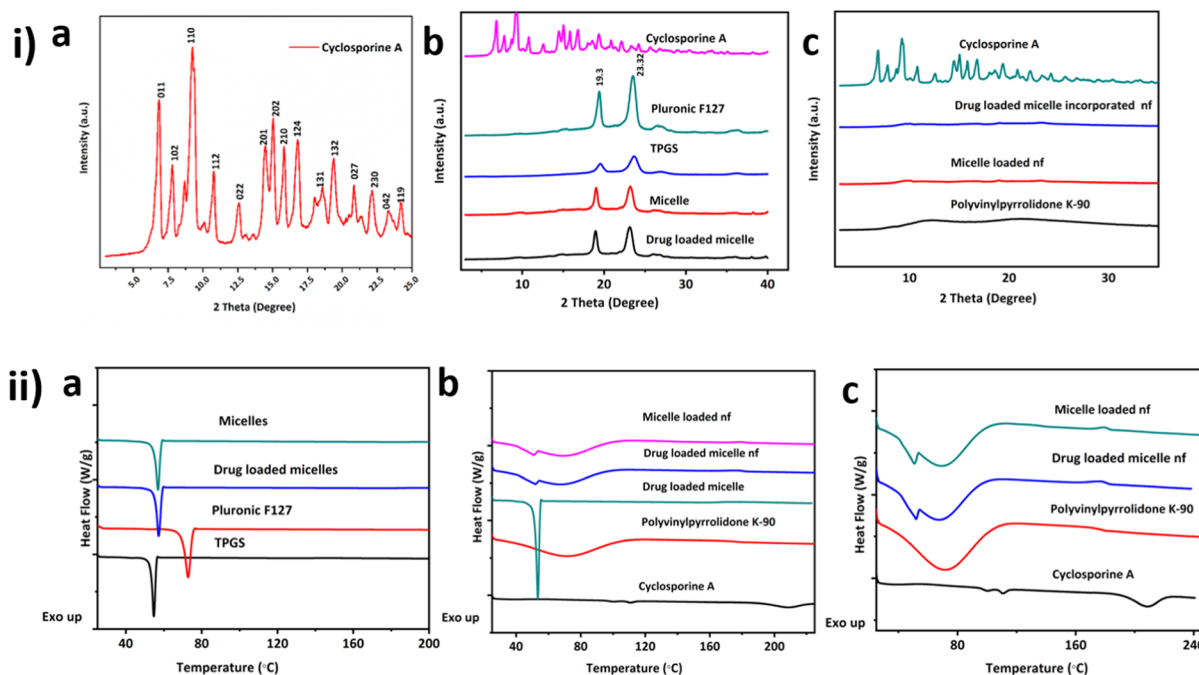
Figure 6. (i) Characteristics powder XRD diffraction patterns of (a) crystalline CyA (b) F127, TPGS, unloaded, and CyA-loaded micelles with the reference to the CyA spectrum (c) PVP, unloaded, and CyA incorporated micelle-loaded nanofibrous system with reference to the CyA spectrum; (ii) DSC data for (a) Pluronic F127, TPGS powder, mixed micelles, and drug-loaded micelles (b) CyA and PVP, unloaded micelles in nanofibers (nf), drug-loaded micelles, drug-loaded micelles in nanofibers, (c) higher resolution DSC data showing transitions for CyA in comparison to formulated systems.
