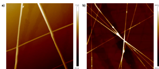
Figure 8. AFM topographic image showing (a) PVP nanofibers and (b) CyA/surfactant-loaded nanofibers; the height scale is included for the two images and a height distribution analysis given in Figure S3.
